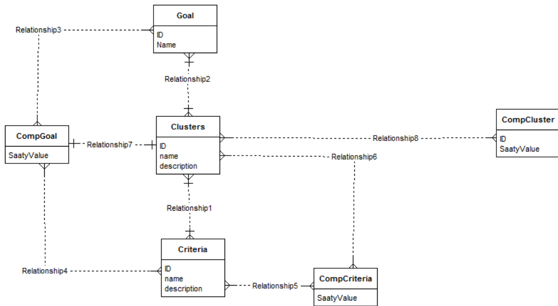
Figure 4. ERA model of the ANP method
