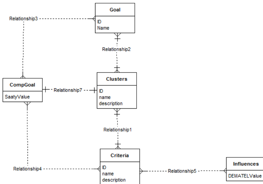
Figure 5. ERA model of the SNAP method
