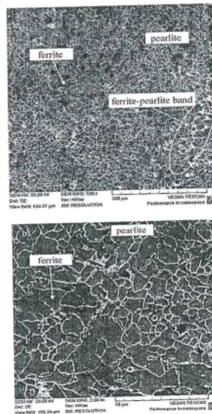
Fig.4. SEM micrographs of sample 1.
