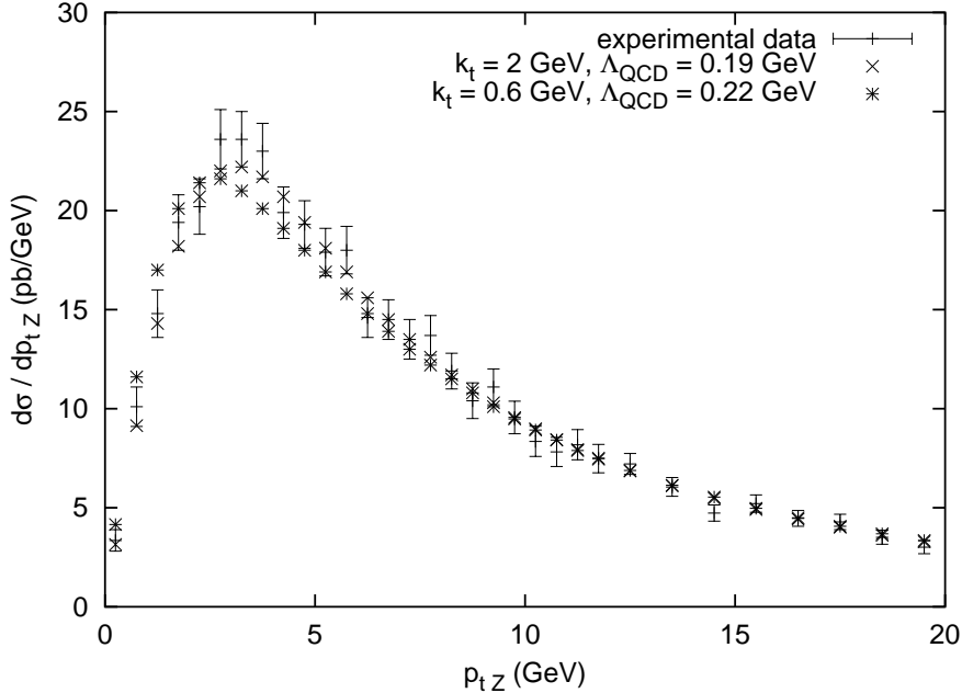
Fig. 1: Comparison of the CDF p_{\perp Z} spectrum with the new shower algorithm for two parameter sets.
