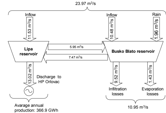
Fig. 3. Water balance of the Orlovac hydroelectric system in 1975-1999 period
