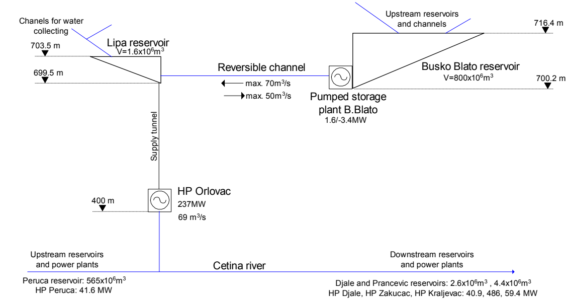
Fig. 2. Orlovac hydroelectric system
