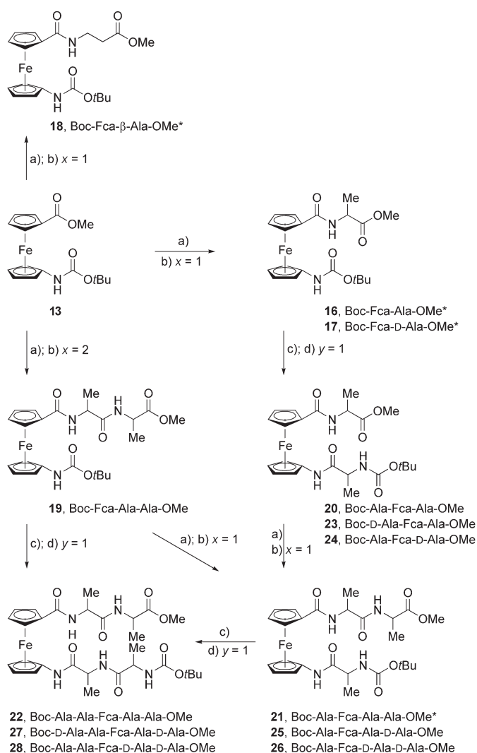
Scheme 3. Syntheses of Fca peptides. a) 1 M \text{NaOH} ; b) 1. EDC/HOBt or HBTU/HOBt, \text{CH}_2\text{Cl}_2 , 2. \text{H}-(\text{Aaa})_x\text{-OMe-HCl}/\text{NEt}_3 , \text{CH}_2\text{Cl}_2 ; c) HCl (gas)/EtOAc or TFA; d) 1. EDC/HOBt or HBTU/HOBt, \text{CH}_2\text{Cl}_2 , 2. Boc-(Aaa) y -OH/ \text{NEt}_3 , \text{CH}_2\text{Cl}_2 . X-ray structures were obtained for compounds marked *.
