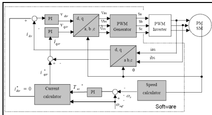
Fig. 3. Block diagram of PMSM speed control system
