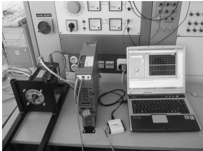
Fig. 4. SM control system with PC, USB DAQ and PWM conv.
