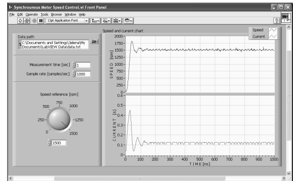
Fig. 6. Motor speed and DC current in LabVIEW Front Panel
