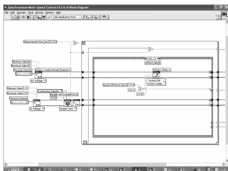
Fig. 5. SM speed control program in LabVIEW Block Diagram
