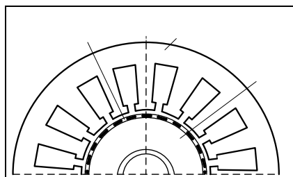
Fig. 1. Cross section of 4 pole synchronous motor with rare-earth permanent magnets mounted on the rotor surface
