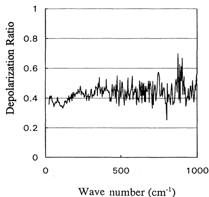
FIG. 4. Depolarization rate of a\text{-GaAs} as a function of wave number: \rho(\omega) = I_{HV}/I_{HH} .
