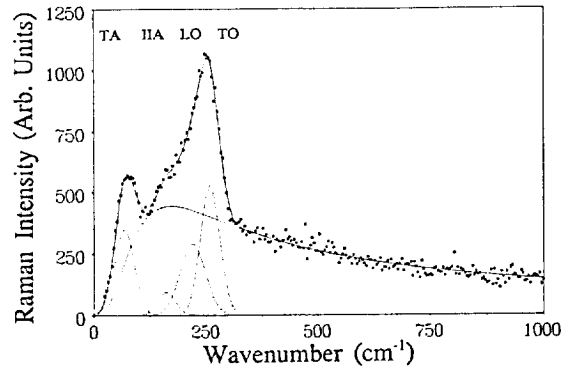
Figure 3. Raman spectrum of GaAs implanted with 3 \times 10^{15} Si/cm 2 . The spectrum is decomposed on the phonon bands and broad background signal (boson peak [2]).
