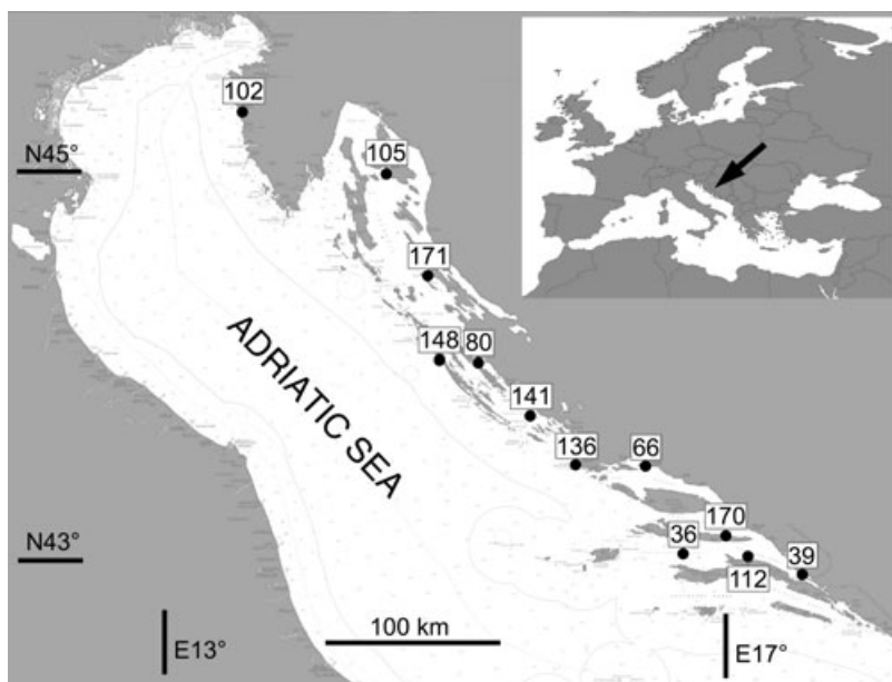
Figure 3. Geographic location of findings of dead bottlenose dolphins with larynx strangulation in the Croatian part of the Adriatic Sea.
