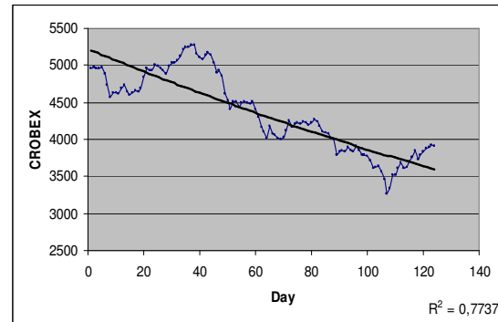
Figure 1 a. CROBEX and approximation by exponential trend.
