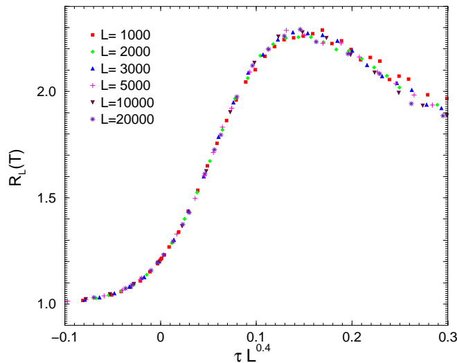
FIG. 2. Ratio R_L(T) for \sigma = 0.9 versus reduced temperature \tau scaled with L^{1/\nu}
