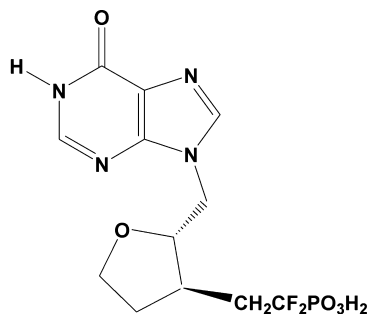
7 (±)-trans-furanyl
