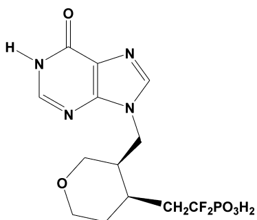
6 (±)-cis-piranyl
