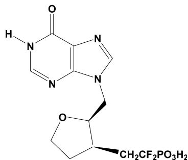
8 (±)-cis-furanyl
