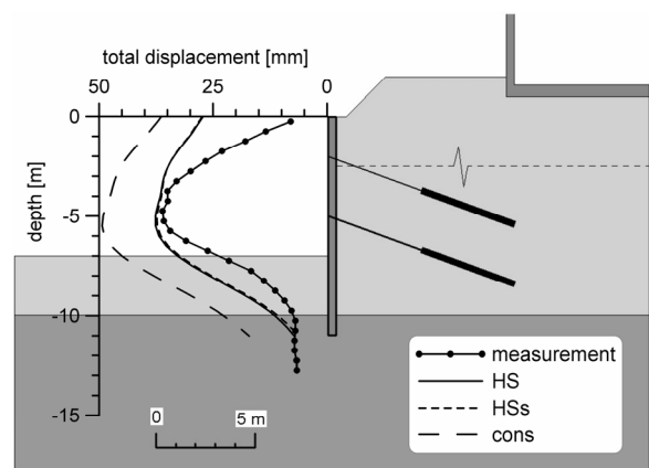
Figure 4 Anchored retaining wall No. 3 at site B: layout and horizontal displacements
