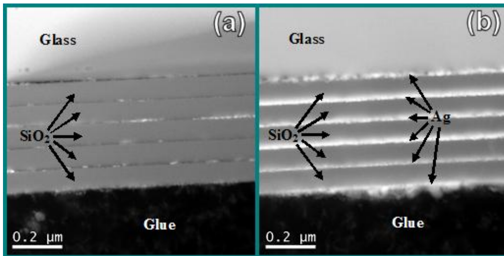
Figure 3: Cross section HAADF STEM micrographs of the EFAD-treated multilayer structure: a) zone A and b) zone B.
