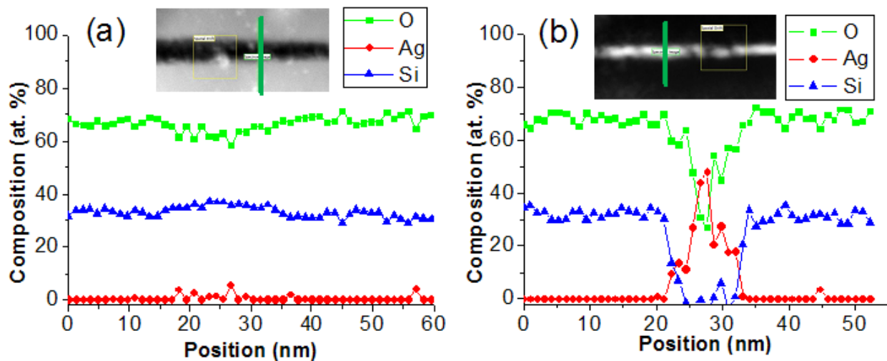
Figure 4: EELS profiles of the zone A (left) and B (right) of the multilayer structure taken around the interface between \text{SiO}_2 films. Inset show STEM micrographs in which EELS spectra were taken (green lines).
