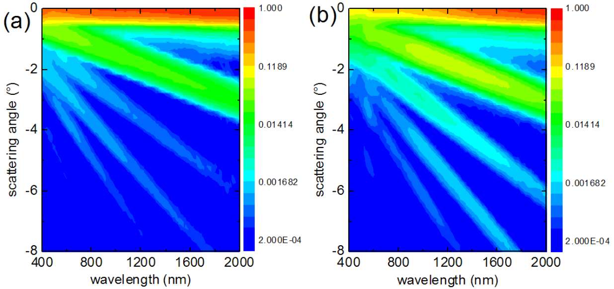
Figure 6: Wavelength-dependence of diffraction pattern of multilayer structures produced by EFAD treatment: (a) multilayer structure \text{BK7}/(\text{Ag}/\text{SiO}_2)^5 with thickness of 7 nm of Ag and 100 nm of \text{SiO}_2 and (b) multilayer structure \text{BK7}/(X/\text{SiO}_2)^5 , in which X represents a multilayer of Ag and \text{SiO}_2 films
