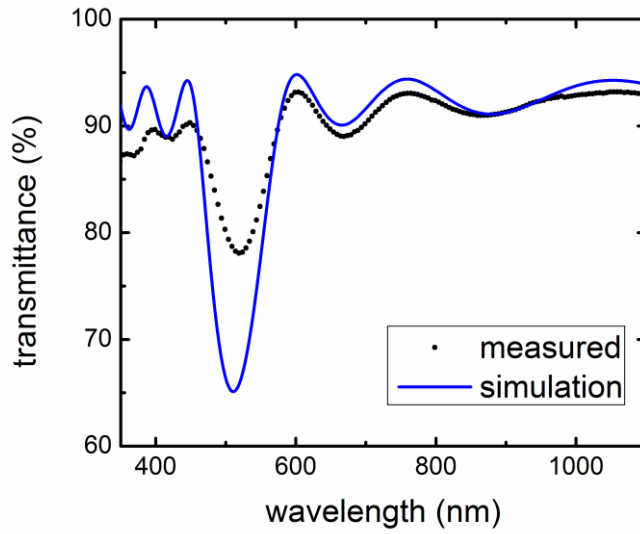
Figure 5: Optical transmittance spectra of zone A of the multilayer structure consisting of substrate/ (X/\text{SiO}_2)^5 , in which X represents a multilayer of Ag and \text{SiO}_2 films (see text for details) after EFAD treatment (black dots) and simulation of an equivalent structure assuming that after EFAD treatment Ag islands are replaced by pores (blue line).
