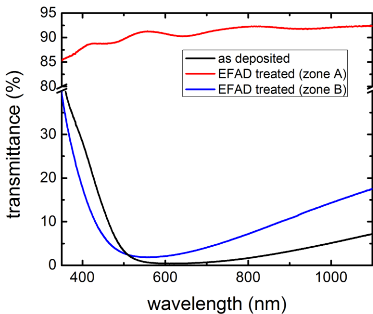
Figure 2: Transmittance spectra of the multilayer structure BK7/(Ag/SiO 2 ) 5 : as deposited sample (black line), zone A (red line) and B (blue line) of the treated sample.
