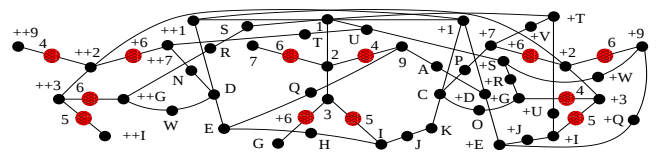
FIG. 6. Conway-Kochen's MMP. Notice that we cannot drop blocks containing ++9, ++I, 7, and G because atoms 4, 5, 6, and +6, from them also share two other blocks each. Why we cannot drop atoms 7, G, H, J, etc., is explained in the text.
