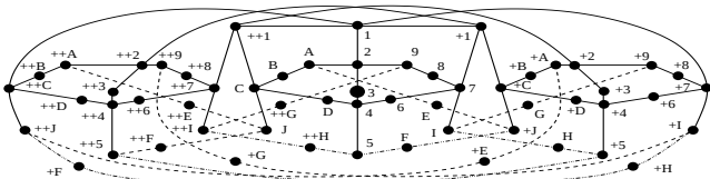
FIG. 4. Peres' KS MMP hypergraph.
