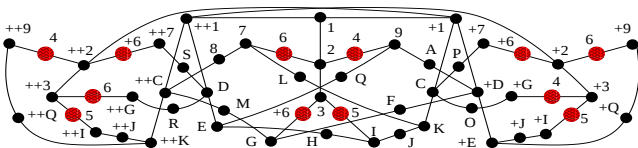
FIG. 5. Bub's MMP with 49 atoms and 36 blocks. Notice that 12 bigger dots with a pattern (red online) represent just 4 atoms: 4, 5, 6, and +6.
