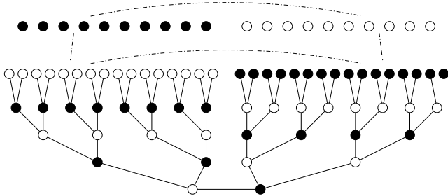
FIG. 10. Starting configuration for generation of 41-41 MMPs
