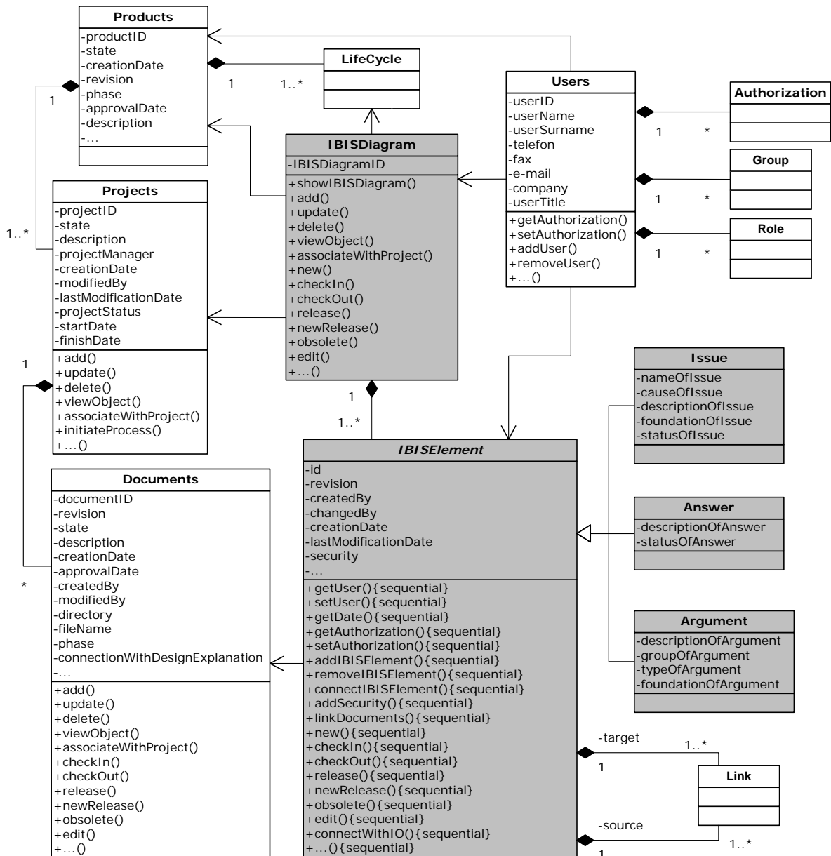
Figure 1. Proposed UML model of IBIS diagrams embedded in PLM system
