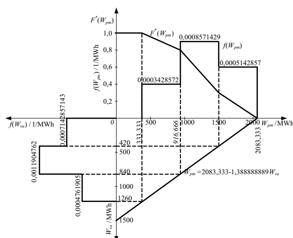
Figure 9 Determination of density function and probability function of required pumping energy
