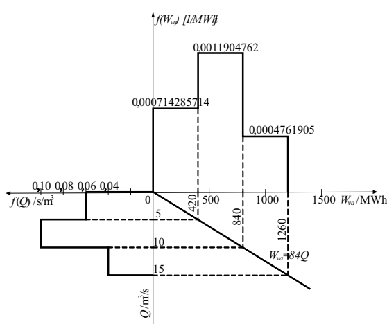
Figure 8 Determination of the density function of variable generation by exclusive usage of natural inflow
