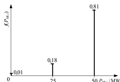
Figure 7 Density function of the outage-dependent plant capacity in turbine drive
