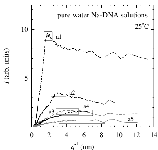
Figure 4. SAXS scattering intensity ( I ) versus inverse wave vector ( q^{-1} ) at T = 25\text{ }^\circ\text{C} of pure water DNA solutions (for DNA concentrations a1-a5 (25, 12.5, 6, 3, 1.6 mg/mL)). Rectangles denote positions and error bars of the peak wave vectors q_m .
