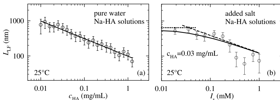
Figure 9. (a) Characteristic length of the LF mode ( L_{LF} ) for pure water HA solutions as a function of HA concentration ( c_{HA} ). The full line is a fit to the power law L_p \propto c_{HA}^{-0.5} . The observed single-chain fundamental length scale corresponds to the renormalized Debye screening length. (b) L_{LF} for HA solutions with varying ionic strength of added salt ( I_s ). The full line is a fit to the the power law L_{LF} \propto I_s^{-0.5} and corresponds to the de Gennes-Dobrynin electrostatic persistence length expected for the flexible chains. (Adapted from ref.9)
