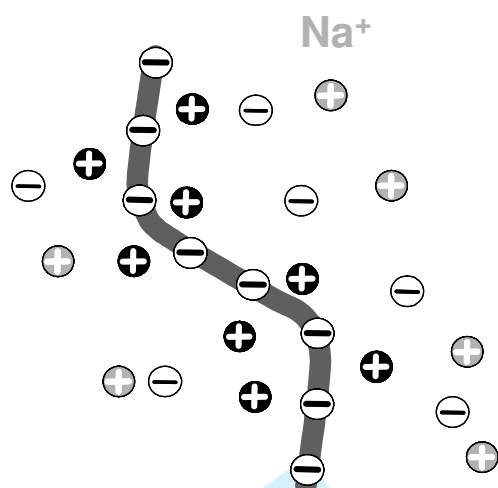
23 24 25 26 27 28 Figure 1. Schematic representation of a (bio)polyelectrolyte: a negatively charged chain is surrounded by a cloud of positive sodium counterions (full symbols). White and gray circles stand for the electrolyte ions in which the biopolymer is dissolved.
