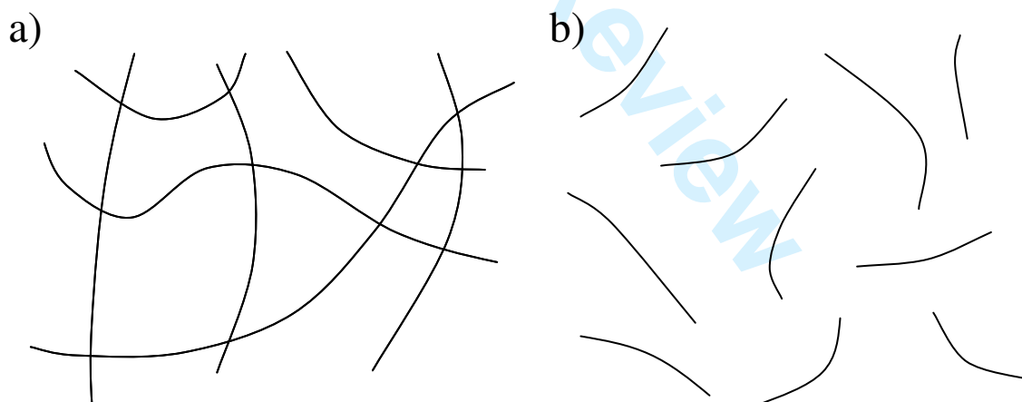
51 52 53 54 55 Figure 2. Long overlapping chains form a semidilute solution (a), whereas short chains or chains at much smaller concentrations are well separated from each other forming a dilute solution (b).
