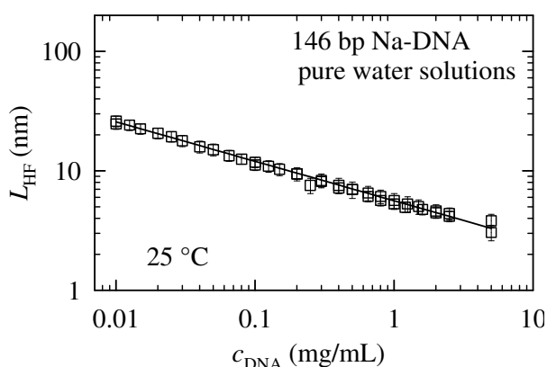
41 42 43 44 45 46 47 48 49 50 51 52 53 54 55 56 Figure 5. Characteristic length of the HF mode ( L_{\text{HF}} ) for pure water 146 bp DNA solutions 57 in dilute regime as a function of DNA concentration ( c_{\text{DNA}} ). The full line is a fit to the 58 power law L_{\text{HF}} \propto c_{\text{DNA}}^{-0.33} . The observed fundamental length scale corresponds to the 59 reduced average distance between chains in dilute regime. (Adapted from ref.5) 60
