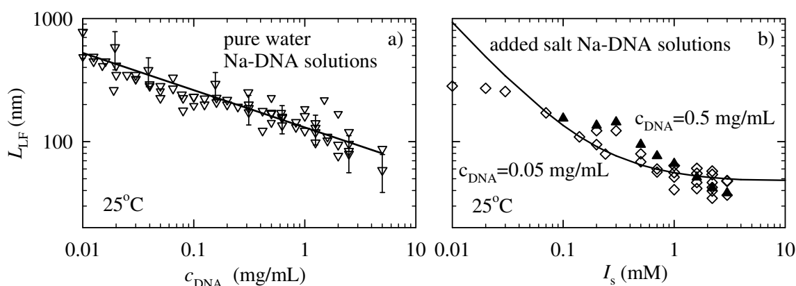
Figure 8. (a) Characteristic length of the LF mode ( L_{\text{LF}} ) for pure water DNA solutions as a function of DNA concentration ( c_{\text{DNA}} ). The full line is a fit to the power law L_{\text{LF}} \propto c_{\text{DNA}}^{-0.25} . The observed single-chain fundamental length scale corresponds to the averaged size of the chain. (b) L_{\text{LF}} for DNA solutions with varying ionic strength of added salt ( I_s ) for c_{\text{DNA}} = 0.05 mg/mL (diamonds) and for c_{\text{DNA}} = 0.5 mg/mL (triangles). The full line is a fit to
