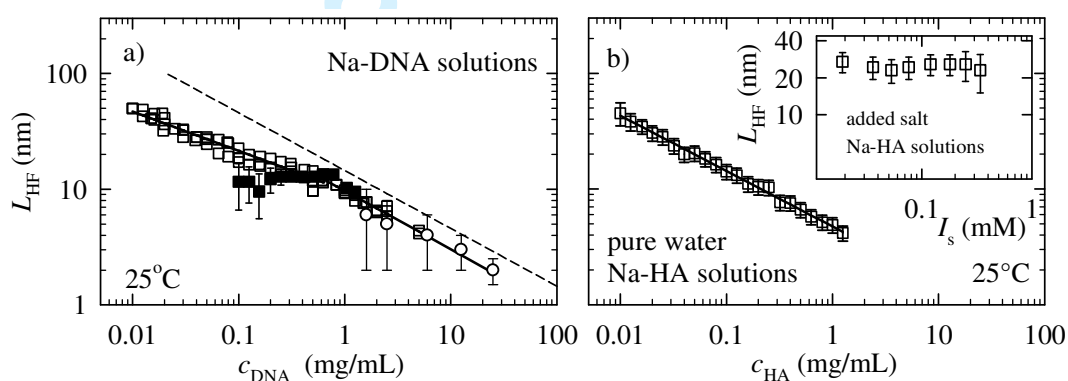
Figure 6. (a) Characteristic length of the HF mode ( L_{\text{HF}} ) for pure water DNA solutions (open squares) and for DNA solutions with added salt I_s = 1 mM (full squares) in semidilute regime as a function of DNA concentration ( c_{\text{DNA}} ). Open circles denote the length scale L \propto q_m^{-1} derived from the SAXS measurements. The full line is a fit to power laws L_{\text{HF}} \propto c_{\text{DNA}}^{-0.33} and \propto c_{\text{DNA}}^{-0.5} at low and high DNA concentrations. The fundamental length scale observed for c_{\text{DNA}} > 0.6 mg/mL corresponds to the semidilute correlation length. The dashed line denotes q_m^{-1} = 14.6 \cdot c^{-1/2} corresponding to the theoretical Koyama prediction for the wormlike chain model. (b) Characteristic length of the HF mode L_{\text{HF}} for pure water HA solutions in semidilute regime as a function of HA concentration ( c_{\text{HA}} ). The full line is a fit to the power law L_{\text{HF}} \propto c_{\text{HA}}^{-0.5} . The observed fundamental length scale corresponds to the semidilute solution correlation length. Inset: L_{\text{HF}} for HA solutions as a function of added salt I_s for a representative HA concentration c_{\text{HA}} = 0.03 mg/mL. (Adapted from ref.4, 6)
