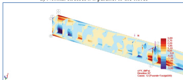
b) Normal stresses y-y perpendicular to the fibres
