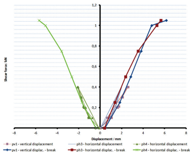
Figure 9 Force/deformation diagram
