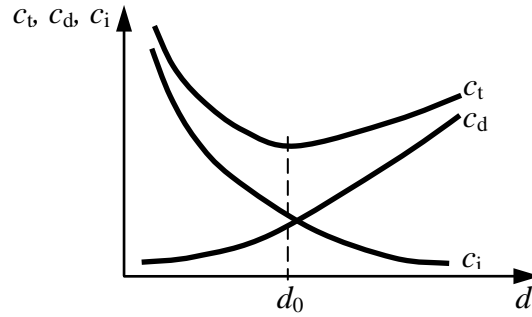
Figure 2. Qualitative representation of total ( c_t ), direct ( c_d ) and indirect ( c_i ) costs related to anti-corrosion protection of a surface, shown as a function of average thickness d of dye covering surface.
