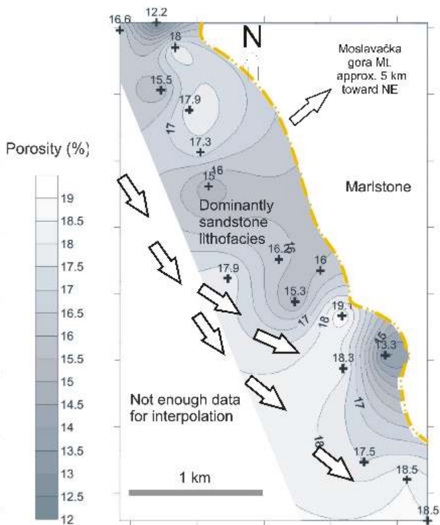
Fig. 12. Ordinary kriging porosity map of the Upper Pannonian reservoir
