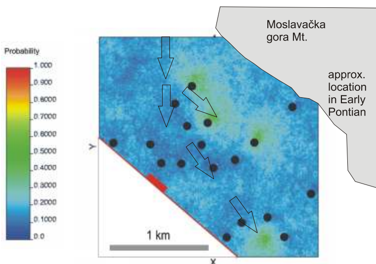
Fig. 11. Probability maps for thickness >13 m – Lower Pontian (modified after Novak Zelenika and Malvi, 2011)
