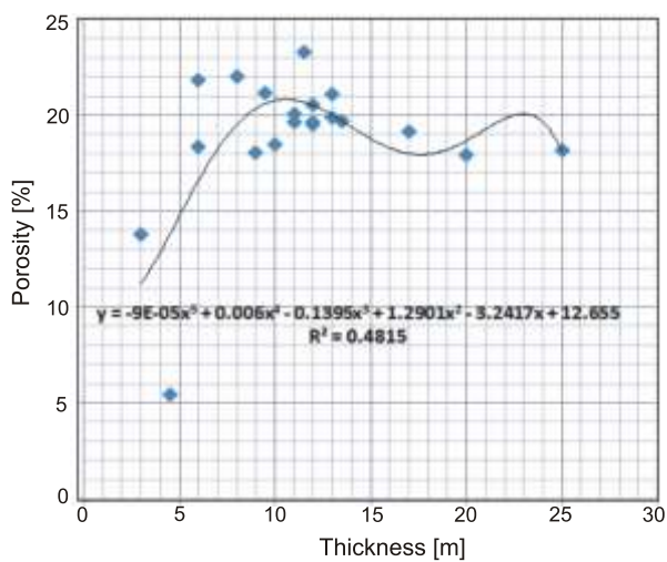
Fig. 5. Thickness vs. porosity based on Lower Pontian reservoir data
