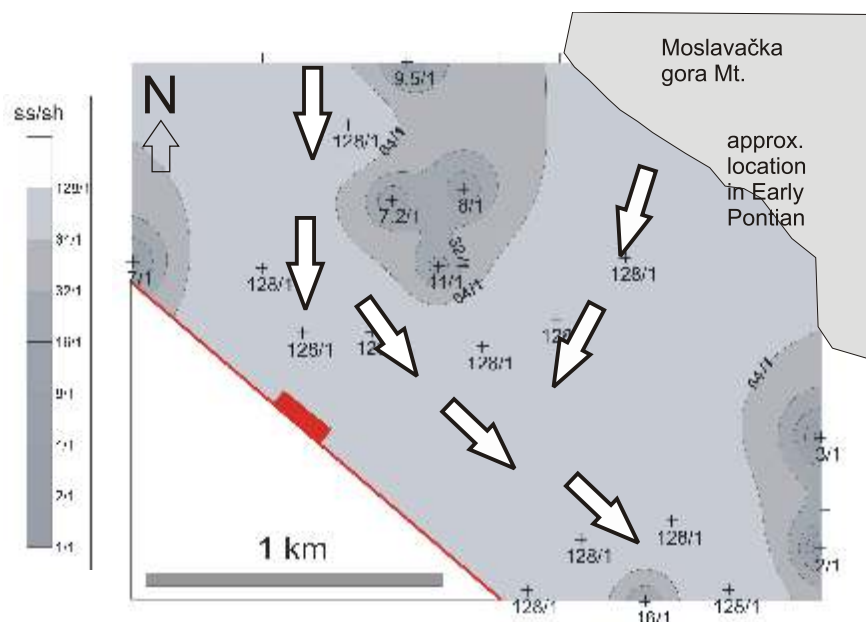
Fig. 17. Ss/sh map of the Lower Pontian reservoir
