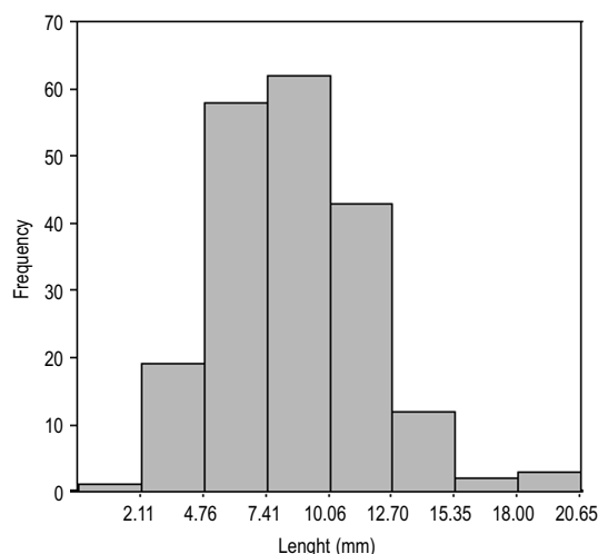
Fig. 3. Information on the geometrical variability of the recycled steel fibres (in terms of length)
