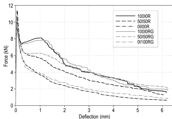
Fig. 10. 28 day splitting tension load – deflection curves
