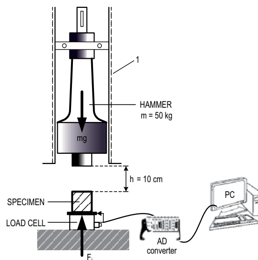
Fig. 7. Layout of the instrumented drop weight system
