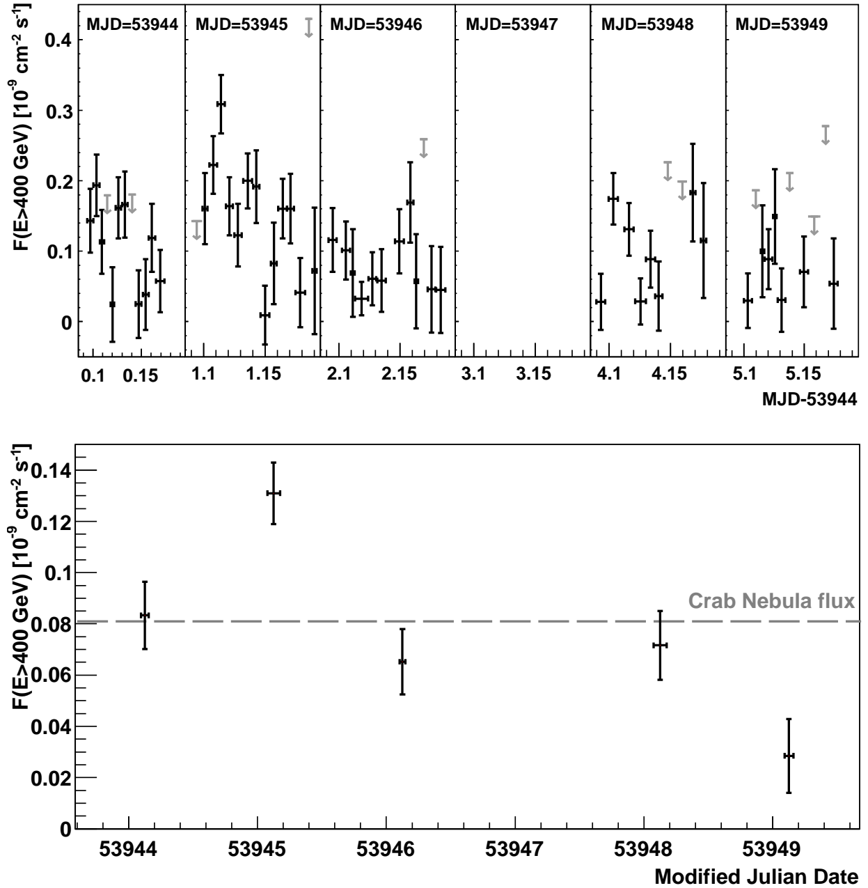
Fig. 7. Top: MAGIC light curve for individual nights for E > 400 \text{ GeV} of PKS 2155-304. Only the second night (MJD 53945) shows significant intra-night variability. Vertical arrows represent flux upper limits at a confidence level of 95%. Bottom: Light curve for the total data set for E > 400 \text{ GeV} with one flux point per night. The error bars in x-direction represent the observation time. The Crab Nebula flux is shown for comparison. For more information see the text.
