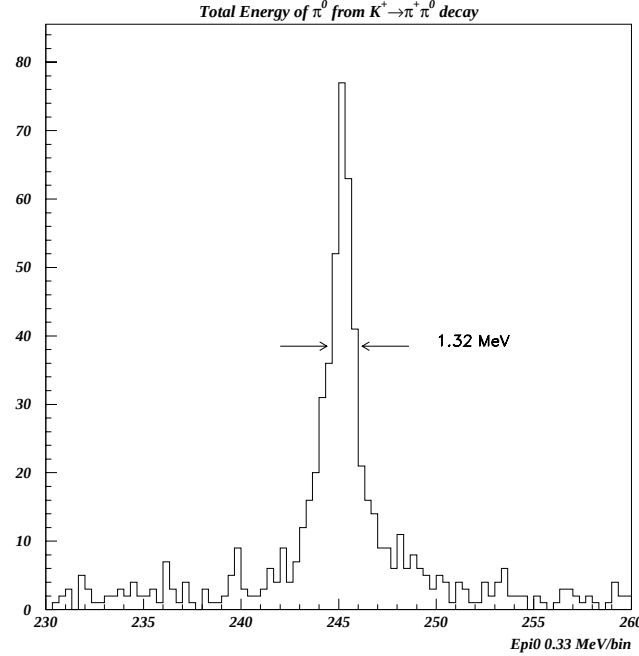
Fig. 2. A spectrum of \pi^0 from the decay, K^+ \rightarrow \pi^0 \pi^+ , showing the NMS resolution.
