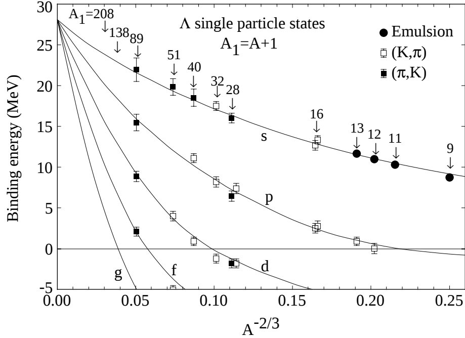
Fig. 1. The binding energy of various hypernuclear shells as a function of A^{-2/3} .
