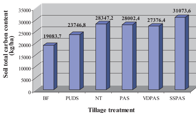
Figure 3. Soil total carbon content in the surface layer (0-30 cm)
