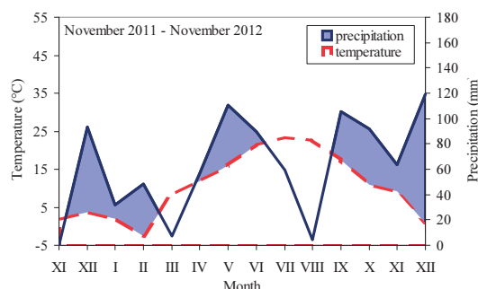
Figure 2. Walter climate diagram for the period November 2011 - November 2012
