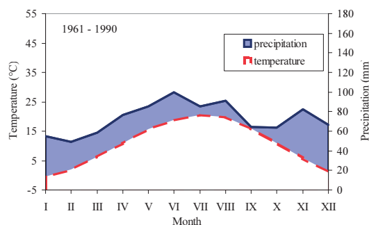
Figure 1. Walter climate diagram for the period 1961 - 1990
