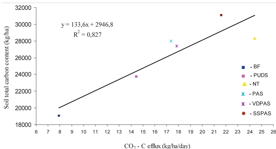
Figure 5. Correlation between soil total carbon content and CO 2 - C efflux
