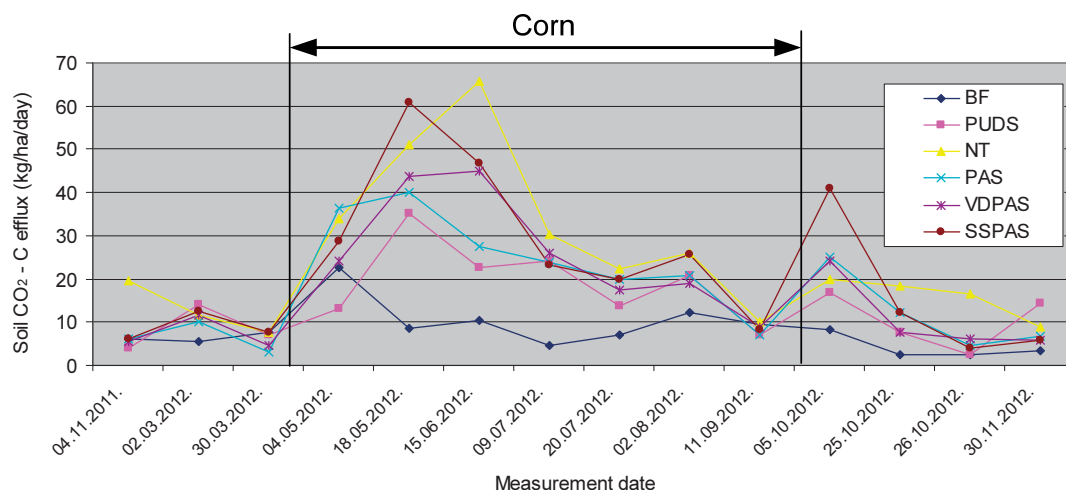
Figure 4. Variations of \text{CO}_2 - C efflux in investigated period
