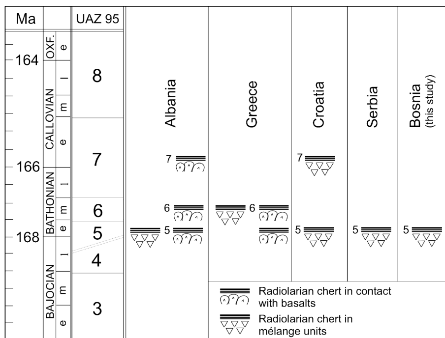
Fig. 5 - Radiolarian age constraints in ophiolite complexes of the Central Dinaridic Ophiolite Belt. Data from the Mirdita Zone, Albania (Chiari et al., 2004), the western ophiolite belt in Greece (Chiari et al., 2003; Bortolotti et al., 2008; Nirta et al., 2010), Croatia (Halamčić et al. 1999), Serbia (Gawlick et al. 2009) and Bosnia (this study). Numerical ages are given according to Gradstein et al. (2012). The UAZ 95 column refers to Unitary Association Zones of Baumgartner et al. (1995b).
