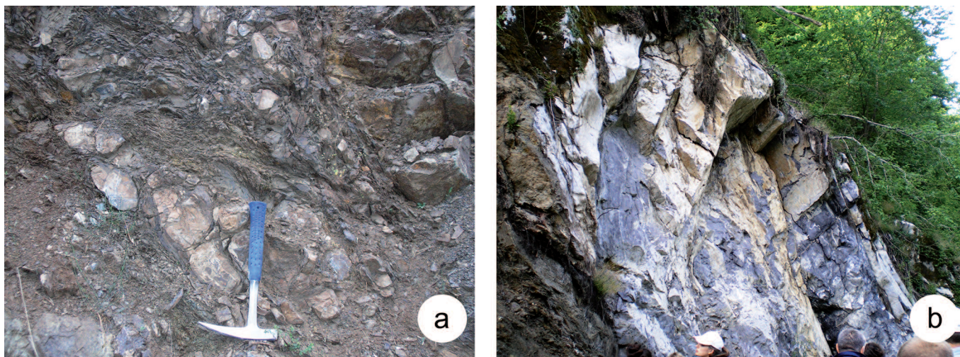
Fig. 4 - a) layered dark grey fine-grained shales with embedded chert blocks; b) the large limestone olistolith that tops the Papratnica section.
