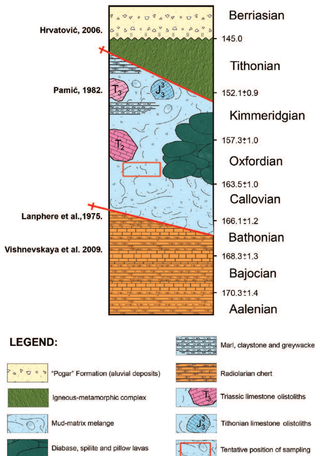
Fig. 2 - Composite stratigraphic section of the Papratnica section. Sampling position indicated within the sequence. Constructed after basic geological map of Yugoslavia, sheet Vareš (Pamić, 1970). Time scale after Gradstein et al. 2012.
