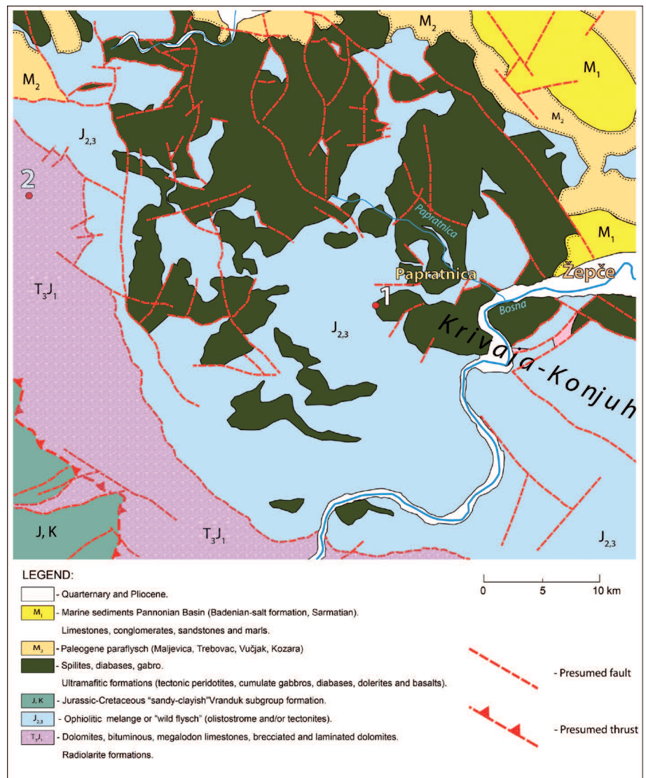
Fig. 3 - Detailed geological map of the sampling area within the western portion of the Krivaja-Konjuh ophiolite complex (KKOC). 1- sampling location, this work; 2- sampling location of the non-ophiolitic chert succession described in Vishnevskaya et al. (2009). Map modified after Jovanović et al. (1978), Pamić (1970), and Dragičević (1987).
