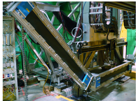
Fig. 23. Two of the eight main detectors, before installation of the lead pre-radiators. The squares standing out on each end of the detectors are lead shielding covering the light guides and PMTs. The quartz sampling scanner is also shown above the lower detector in the figure.
