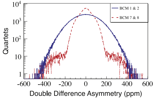
Fig. 9. Charge asymmetry double difference plots for two pairs of BCMs from a typical 1 h run. The DD 12 (broad curve) has an RMS width of 115 ppm. The DD 78 (skinny curve with shoulders) has an RMS width of only 57 ppm.
