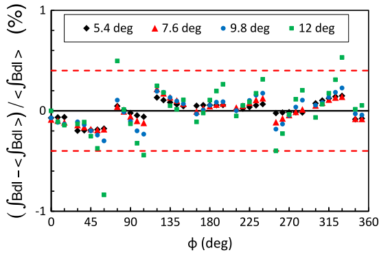
Fig. 22. Relative difference (\langle f B dl \rangle - \langle f B dl \rangle) / \langle f B dl \rangle between the eight-octant average \langle f B dl \rangle and the calculated f B dl for each octant based on the actual coil positions as determined from the zero-crossing field mapping measurements. The results for each octant are plotted as a function of the azimuthal angle \phi for the four different polar angles \theta indicated in the legend. \phi=0 corresponds to the center of the top octant, and increases going clockwise around the beam axis. The dashed lines indicate the specification on this parameter. Note that the smallest and largest polar angles plotted are just outside the scattered electron acceptance defined by the collimation system. The same is true for the azimuthal range.
