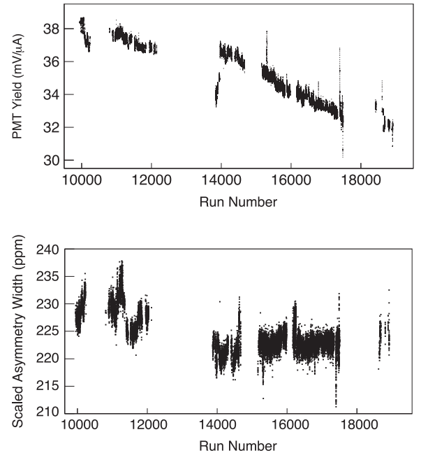
Fig. 25. Top: typical charge normalized main detector phototube yields over the course of the experiment. Run 2 started around run 14,000. The \sim 10\% decrease in yield over time is attributed to gain degradation. The change at run 14,000 corresponds to a period when the beam current was raised as Run 2 got underway. Spikes near runs 15,500 and 17,500 are the results of temporary issues with heat dissipation in the BCM and DAQ electronics, respectively. Bottom: The main detectors' asymmetry width over the whole experiment, scaled by \sqrt{l/180} , where l is the beam current in \mu A. As described in the text, this metric combines detector, target, and BCM performance as well as regression to correct for HCBA.
