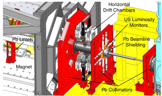
Fig. 26. A CAD drawing of the triple collimation region. The target is in the scattering chamber on the right side of the drawing; the beam direction is to the left. The lead collimators and the lead lintels between the magnet coils are shown in this view. The horizontal drift chambers are shown just upstream of the third collimator. The four upstream luminosity monitors are shown mounted to the upstream face of the middle collimator, each with two light guides and PMTs. The active elements span the light guide pairs in the horizontal and vertical octants.
