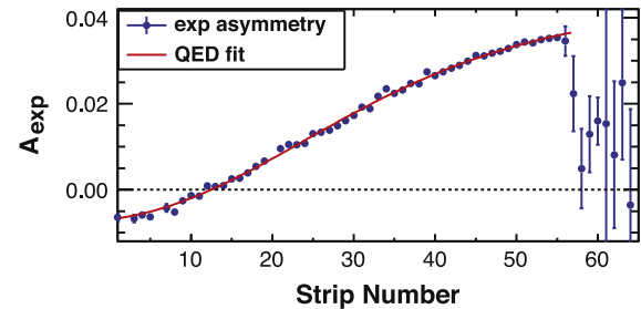
Fig. 14. A spectrum of the measured asymmetry for each strip along with the fit to a QED calculation shown by the solid line. The three missing strips, out of the > 50 active strips, have a negligible impact on the quality of the fit and the extracted electron polarization.
