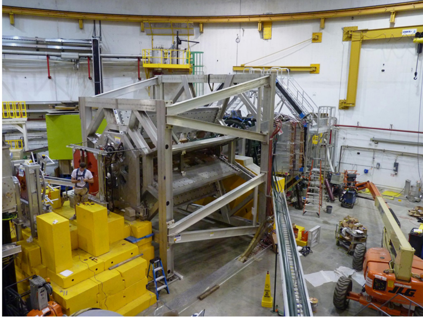
Fig. 2. The Q_{\text{weak}} experimental apparatus during installation, before most of the equipment was covered with shielding. The target scattering chamber is on the left, followed by the first two lead collimators on either side of the man in the figure. A third lead collimator faced with aluminum sits just in front of the large frame in the center of the picture, which supports the eight magnet coils. Three of the eight quartz detector bars appear just downstream and to the right of the magnet as skinny, long bars.
