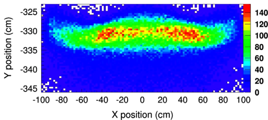
Fig. 31. A projection of tracks found in the VDCs to the main quartz detector in the bottom octant. The trigger used for these events did not include the 2\text{ m} wide main detector itself, which extended from -326\text{ cm} to -344\text{ cm} in Y . The X -axis is in horizontal direction, the Y -axis is in vertical direction. The scale indicates the relative electron flux.
