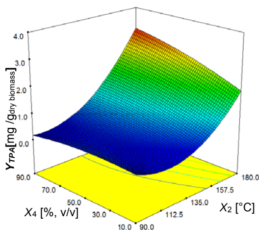
Figure 2: 3D graphics surface of TPA as a function of extraction temperature ( X_2 ) and ethanol concentration ( X_4 ) at fixed time (80 min) and liquid - solid ratio (15 mL/g) as for corn silage
