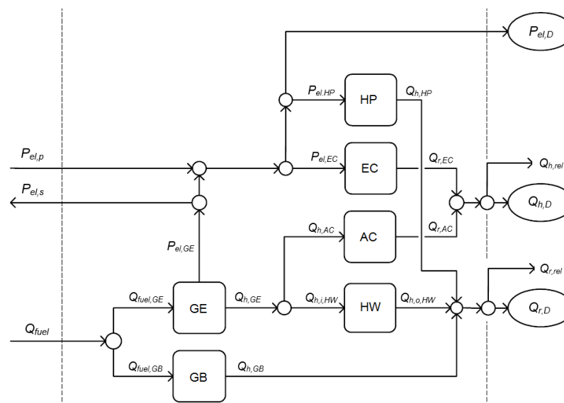
Figure 1. Small-scale CHCP system scheme
