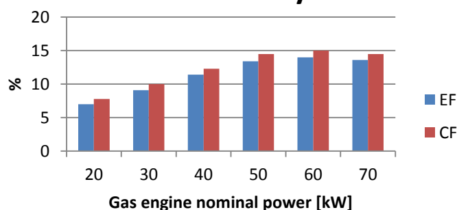
Figure 18. Savings factors for different gas engine nominal power – Cost energy optimization-summer day
