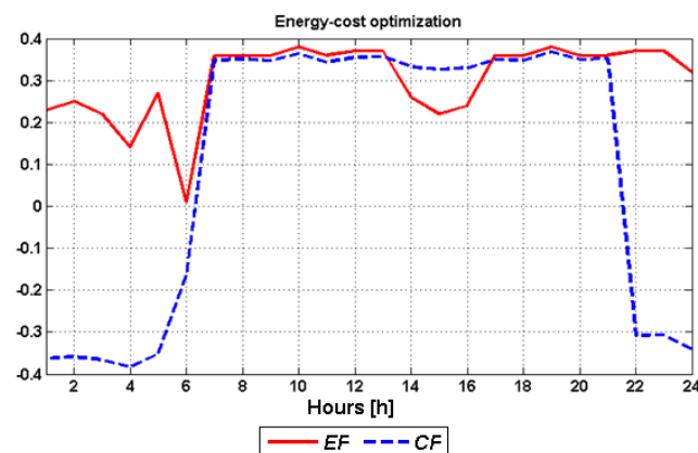
Figure 8. Savings factors-winter day energy-cost optimization
