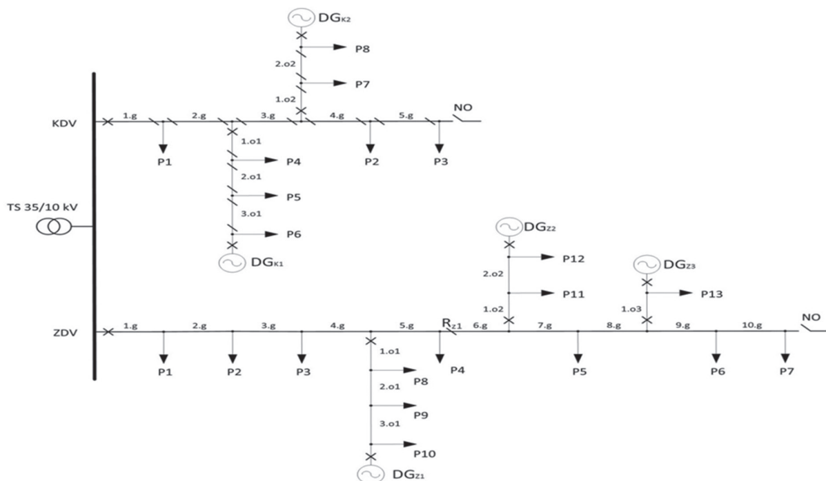
Fig. 2. Single-line network diagram - second case
