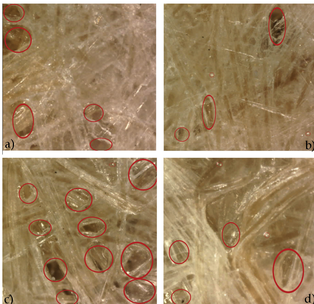
Figure 11 Dino-Lite digital microscope images at 50× magnification presenting voids on the surface of: (a) CR composite; (b) C1 composite; (c) C2 composite; and (d) C3 composite.
