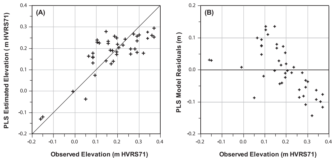
FIGURE 6. Scatter plot from a screened PLS transfer function (component 2) showing observed versus predicted elevation (A) and residual values versus observed elevation (B).
