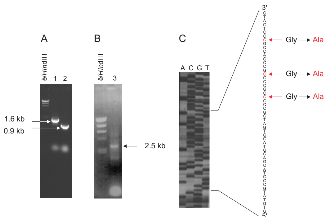
Fig. 8. Site-directed mutagenesis of the cloned otcC gene; two PCR products (A), their combination (B) and partial DNA sequence (C) are shown replacing three guanines by three cytosines in order to change three glycines, in the enzyme active site, into three alanines
