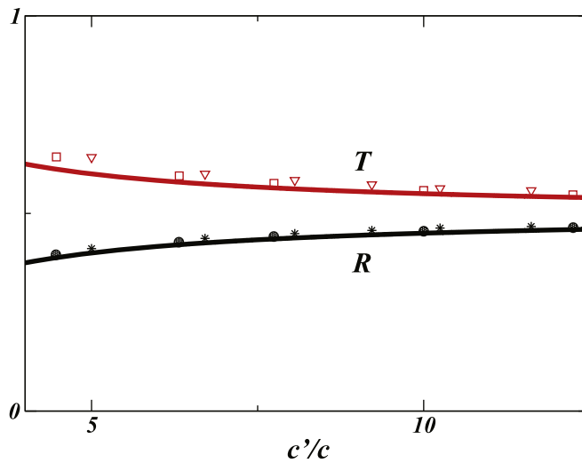
Figure 4. Points are values of R (filled black circles for V = 0.96c and black stars for V = 0.9c ) and T (empty red squares for V = 0.96c and red triangles down for V = 0.9c ) versus c'/c numerically computed from the GP equation. Solid lines are the analytical predictions (53), (54) for R and T .
