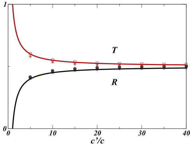
Figure 10. Plot of R (bottom black) and T (top red) for the quenched Calogero model showing the height of the reflected and transmitted peaks as seen from numerics and their comparison with analytical calculations (equation (73)). Points are numerical results: filled black circles (black stars) are the values of R for \nu = 0.04 ( \nu = 0.07 ), while empty red squared (red stars) are the corresponding values for T again for \nu = 0.04 ( \nu = 0.07 ).
