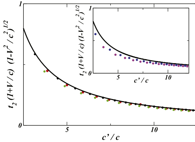
Figure 7. Plot of t_2 times (1 + V/c) \cdot \sqrt{1 - V^2/c^2} as a function of c'/c ; dots are from the numerical solution of the GP equation for V/c = 0.96 (black), 0.9 (red), 0.75 (green) with c = 1 , while the solid line is the analytical prediction (69). Inset: same plot for V/c = 0.6 (blue) and 0.4 (magenta).
