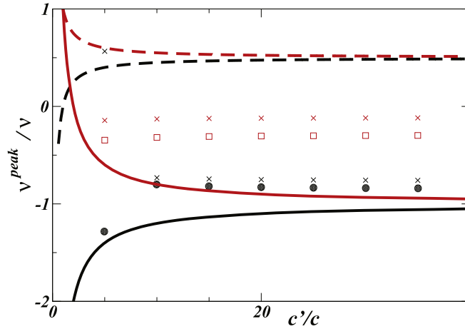
Figure 9. Plot of the reduced peak velocity in units of \nu as obtained from the numerics: filled black circles (black stars) are the values of reflected peak velocities for \nu = 0.04 ( \nu = 0.07 ), while empty red squared (red stars) are the corresponding values for transmitted peak velocity for \nu = 0.04 ( \nu = 0.07 ). Solid lines corresponds to the analytical predictions (74) and (75), respectively for the reflected (black) and transmitted (red) peak velocities. Dashed lines are the predictions for the bulk reflected (black) and transmitted (red) bulk velocities according to (73).
