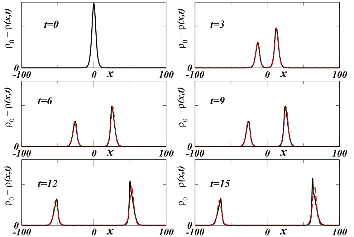
Figure 8. Plot of the density \rho_0 - \rho(x, t) of the moving bump for the different times t = 0, 3, 6, 9, 12, 15 for g' = 20 and V/c = 0.96 (here t_0 = 0 ). The solid black lines are numerical results from the GP equation, while the red dashed ones (of course not plotted at the initial time) are from the analytical prediction (13). For the considered parameters it is t_2 \approx 0.728 and t_3 \approx 15.749 .
