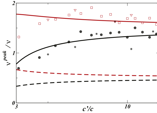
Figure 3. Points are reduced peak velocities in units of v versus c'/c numerically computed from the GP equation: filled black circles ( V = 0.96c ) and black stars ( V = 0.9c ) are the reflected velocities, empty red squares ( V = 0.96c ) and red triangles down ( V = 0.9c ) are the transmitted ones. Solid lines are the analytical predictions (55), (56) for the reflected (black) and transmitted (red) reduced peak velocities, while the dashed lines are the analytical predictions (53), (54) for the reflected (black) and transmitted (red) reduced bulk velocities.
