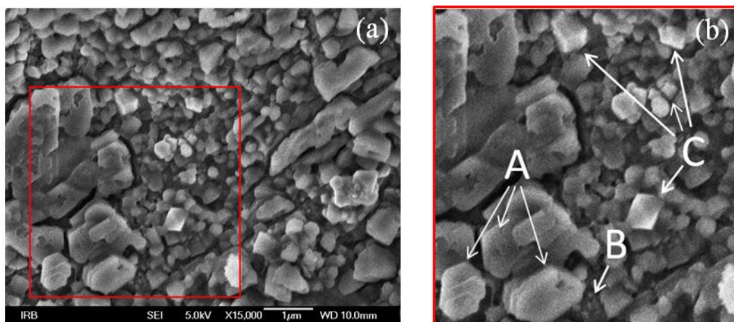
Figure 4. FE-SEM micrograph of the Sample 2, shown in (a). The magnified region of the sample from the marked red square in (a), shown in (b), reveals three different morphologies present in the sample: hexagonal shapes (A), spherical particles (B) and shapes like prisms (C).
