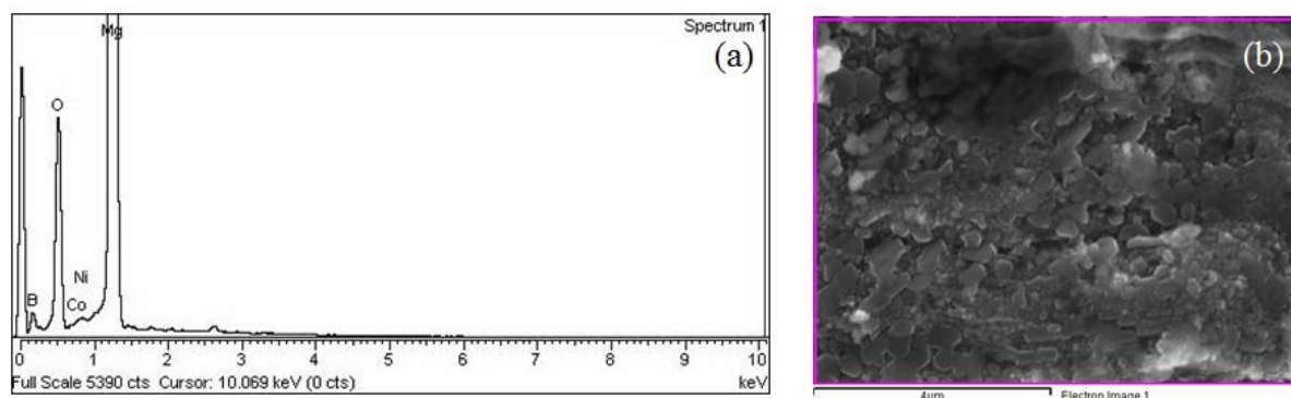
Figure 7. EDS spectrum of the Sample 1 (a), taken from a region of the sample shown in (b).
