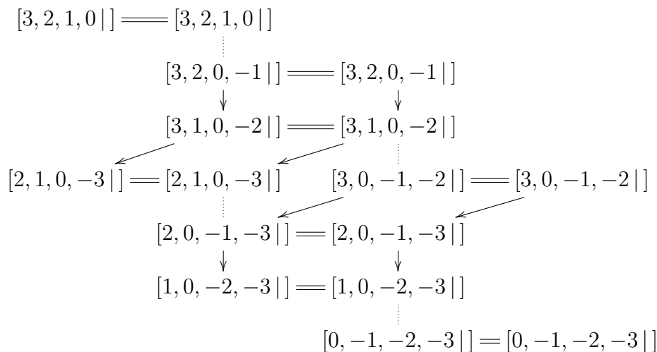
Figure 5.4: Singular orbit for \Sigma = \{\alpha_4\} , \lambda + \rho = [3, 2, 1, 0]
