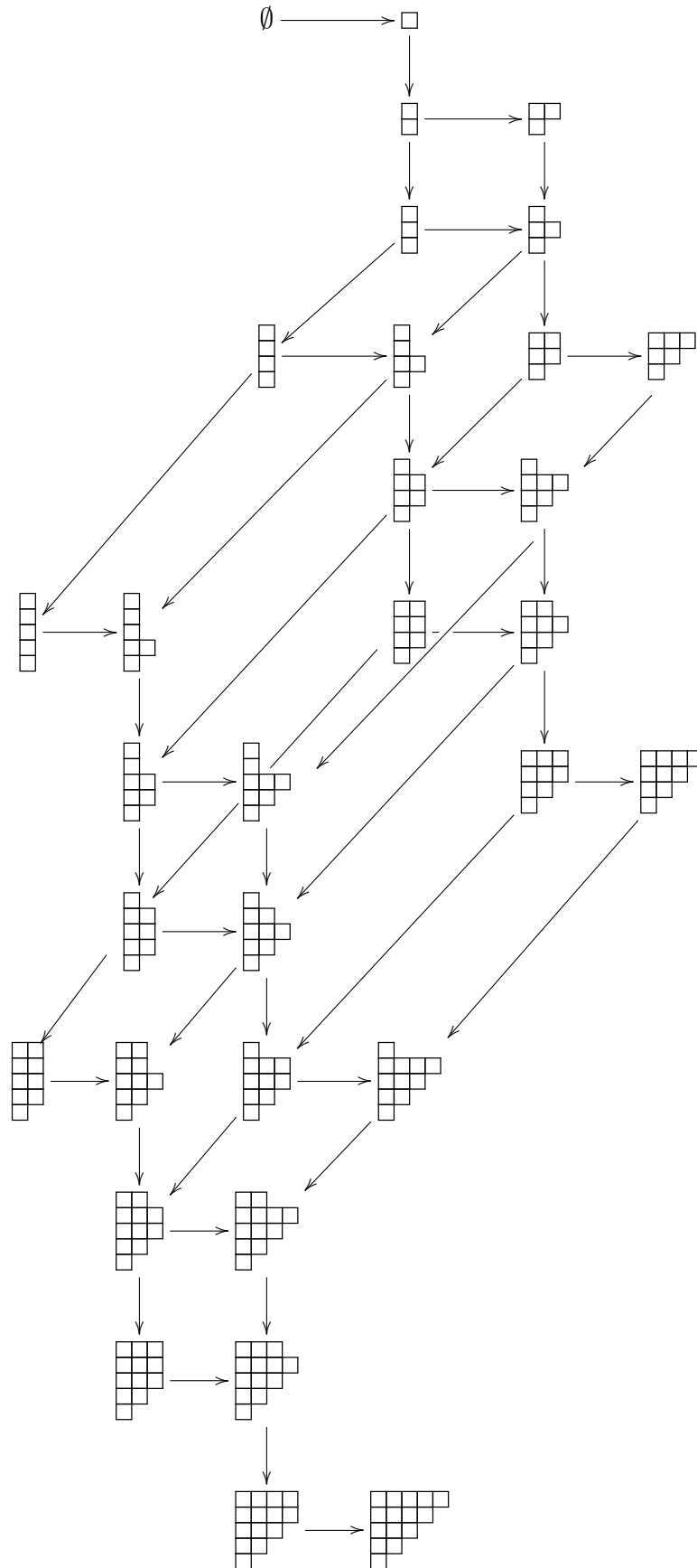
Figure 4.5: W^p for p = 0-1-2-3-4
