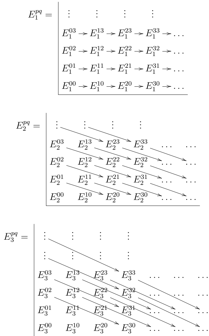
Figure 1.2: First three pages of a first quadrant spectral sequence
