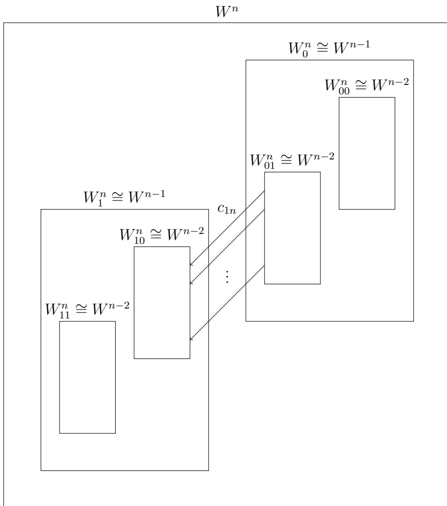
Figure 4.6: Inductive structure of W^{\mathfrak{p}} for \mathfrak{p} = \circ - \circ \cdots \circ - \circ \leftarrow \times
