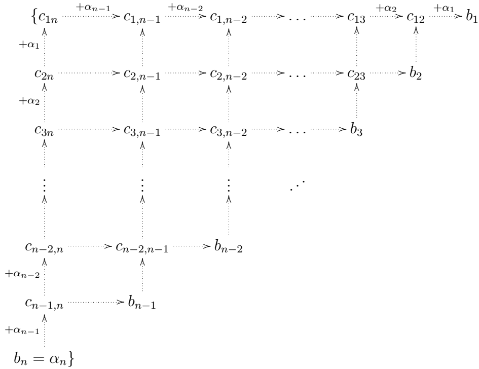
Figure 4.1: \Delta(\mathfrak{u}) for \mathfrak{p} = \circ - \circ - \dots - \circ - \circ \leftarrow \times
