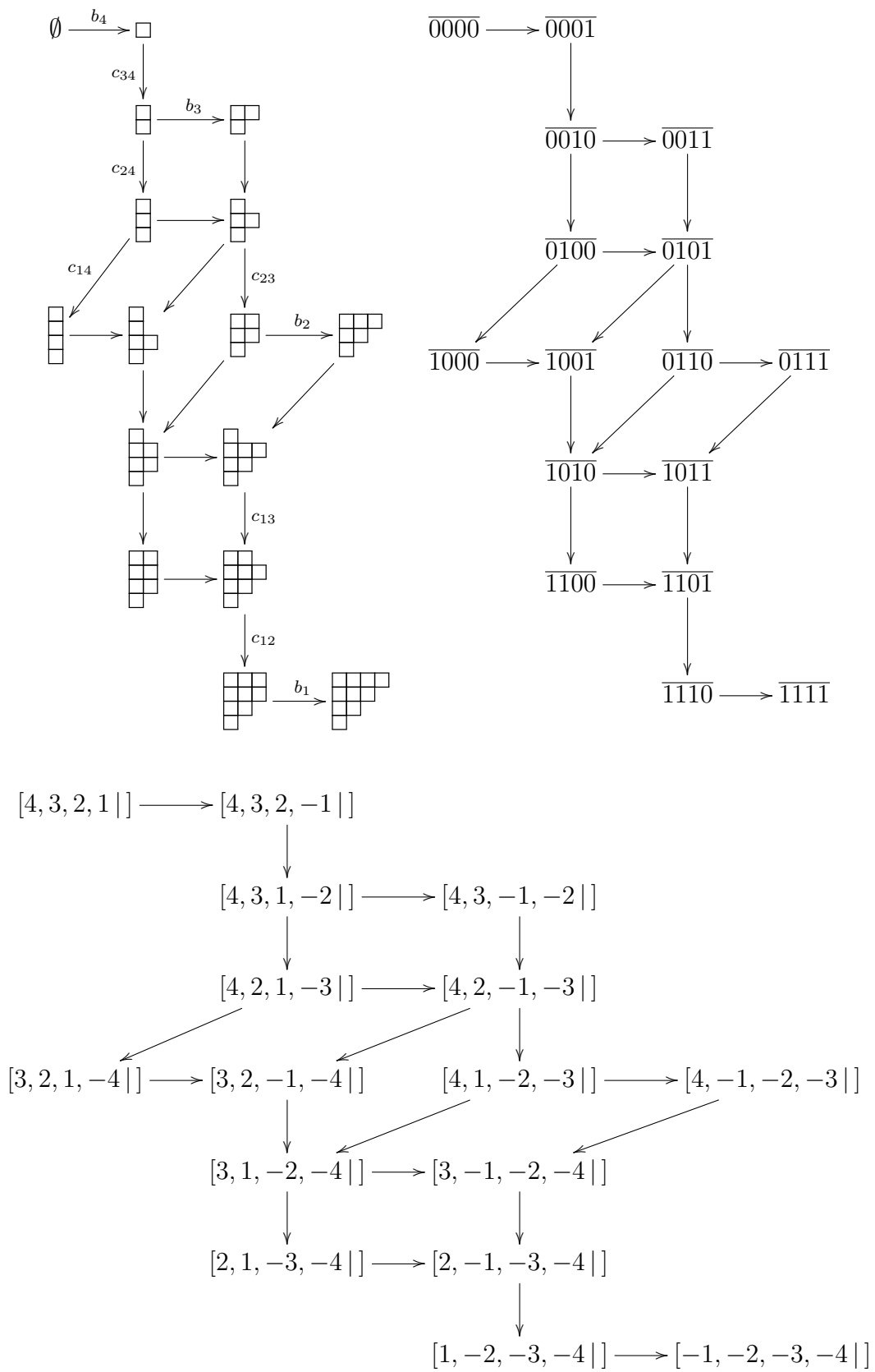
Figure 4.4: W^p and W^p \rho for p = o-o-o-lx
