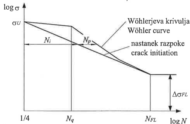
Sl. 1. Shematska predstavitev dobe trajanja strojnih elementov Fig 1. Schematic representation of the service life of machine elements
