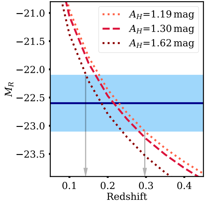
Figure 4. Expected rest-frame R -band absolute magnitude of the host galaxy HESS J1943+213 as a function of redshift (see Section 4 for details). Dashed and dotted lines show the effect of different level of dust extinction. The average M_R of BL Lac host galaxies derived by Sbarufatti, Treves, & Falomo (2005b) is shown as a horizontal blue line, with the \pm 1\sigma regime highlighted in light blue. The redshift of HESS J1943+213 is thus constrained in the range 0.14 \lesssim z \lesssim 0.30 (vertical grey arrows).
