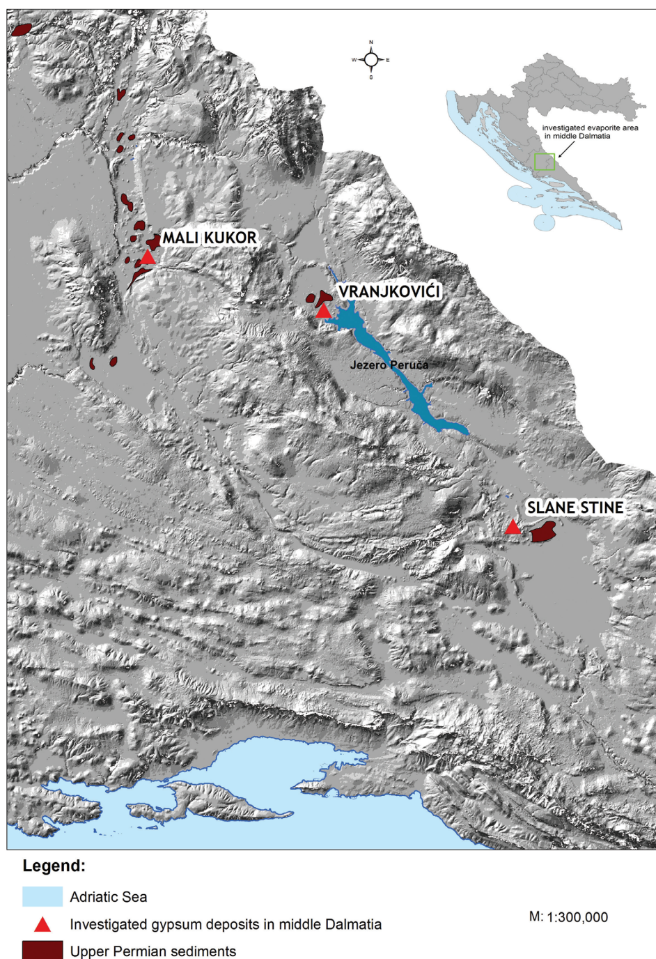
Figure 1. Map to show the locations of the study sites in middle Dalmatia, Croatia. The reference source for Upper Permian sediments used in this paper is the 1:300,000 Geological Map of the Republic of Croatia (CGS, 2009).
