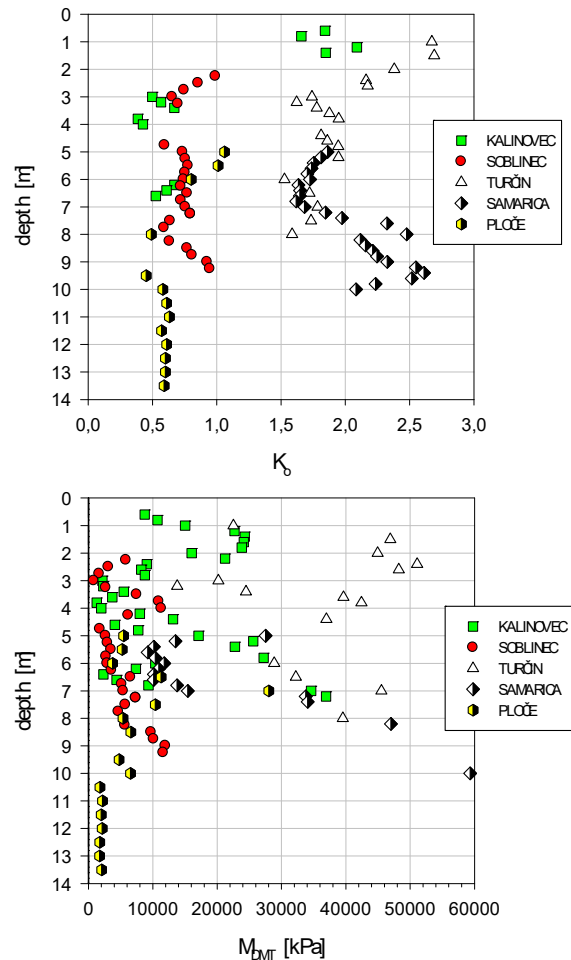
Fig. 6 DMT for the horizontal stress index ( K_0 ) and the oedometer modulus ( M_{DMT} )
