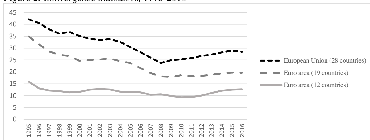
Figure 2. Convergence indicators, 1995-2016
