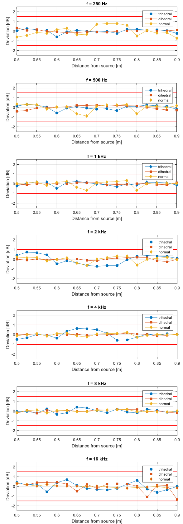
Figure 1. Deviations from the free-field decay (ISO 3745 estimate) versus distance from the source.
