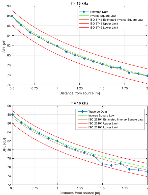
Figure 4. Inverse square law performance at 16 kHz for ISO 3745 and ISO 26101
