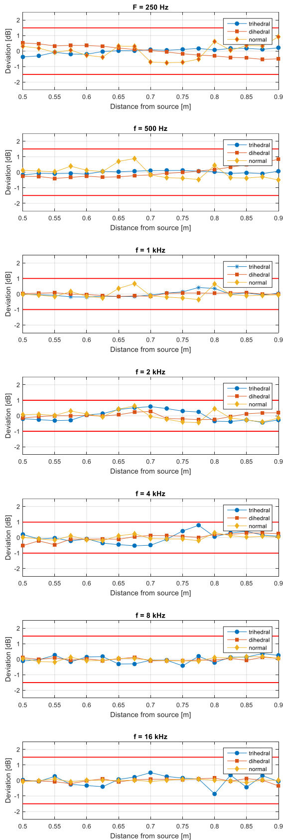
Figure 2. Deviations from the free-field decay (ISO 26101 estimate) versus distance from the source.
