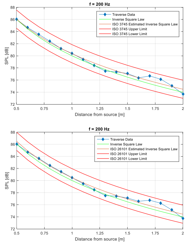
Figure 3. Inverse square law performance at 200 Hz for ISO 3745 and ISO 26101
