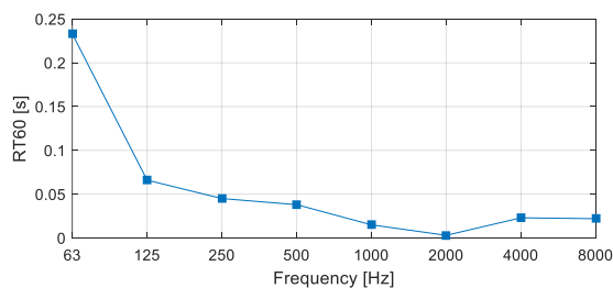
Figure 5. RT60 reverberation time in octave bands
