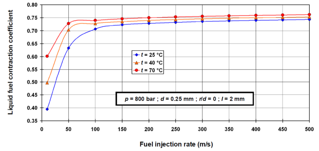
Fig. 2. Change in liquid fuel contraction coefficient for different fuel injection rates and temperatures ( p = 800 \text{ bars} )
