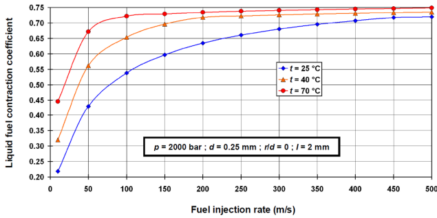
Fig. 4. Change in liquid fuel contraction coefficient for different fuel injection rates and temperatures ( p = 2000 bar)
