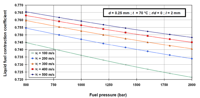
Fig. 8. Change in liquid fuel contraction coefficient for different fuel pressures and injection rates ( t = 70 °C)
