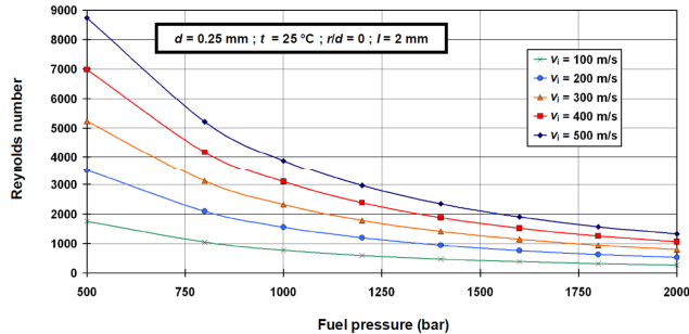
Fig. 9. Change in Reynolds number for different fuel pressures and injection rates ( t = 25\text{ }^{\circ}\text{C} )
