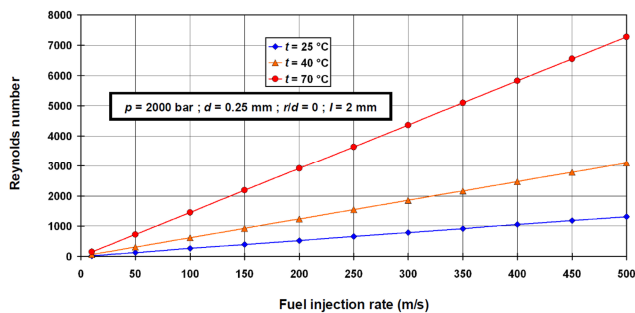
Fig. 5. Change in Reynolds number for different fuel injection rates and temperatures ( p = 2000 bar)
