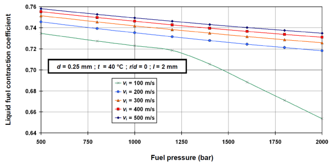
Fig. 7. Change in liquid fuel contraction coefficient for different fuel pressures and injection rates ( t = 40 °C)
