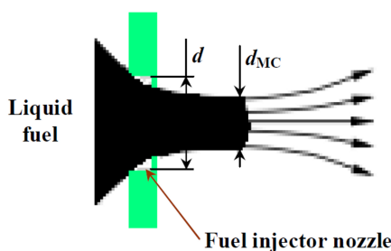
Fig. 1. Liquid fuel contraction coefficient definition for fuel injector nozzle
