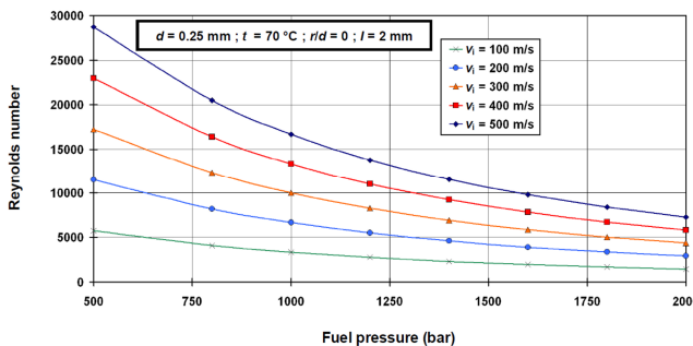
Fig. 10. Change in Reynolds number for different fuel pressures and injection rates ( t = 70\text{ }^{\circ}\text{C} )
