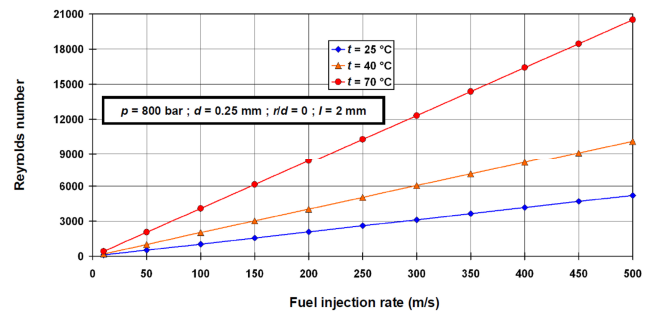
Fig. 3. Change in Reynolds number for different fuel injection rates and temperatures ( p = 800 \text{ bars} )
