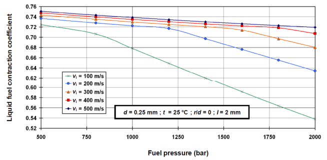
Fig. 6. Change in liquid fuel contraction coefficient for different fuel pressures and injection rates ( t = 25 °C)
