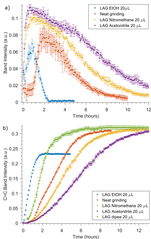
Fig. 4 a) Formation kinetics and life-span of barb:van cocrystal in neat grinding and LAG reactions, derived from cocrystal Raman band at 1735 \text{ cm}^{-1} , and b) kinetics of C=C bond formation derived from changes in intensities of the band at 1542 \text{ cm}^{-1} . LAG with EtOH yielded III while other liquids yielded I . The intensity of the C=C band is lower in III than in I . Note the different scales in a) and b).
