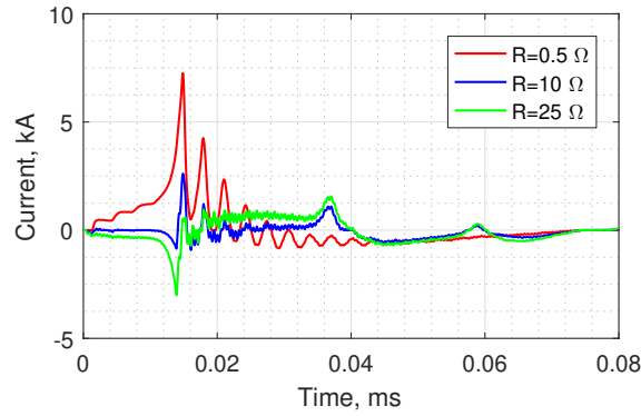
Fig. 10. Comparison of currents conducted by the SPD in phase C at the LV transformer side, for grounding resistances 0.5 \Omega , 10 \Omega and 25 \Omega
