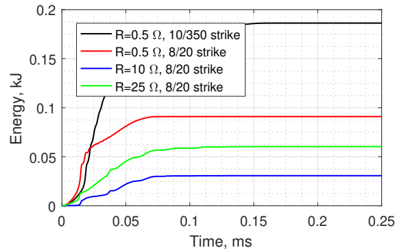
Fig. 12. Energy absorption of the SPD in phase C at the LV side of the transformer, for 8/20 \mu s and 10/350 \mu s lightning wave-shapes and grounding resistances 0.5 \Omega , 10 \Omega and 25 \Omega
