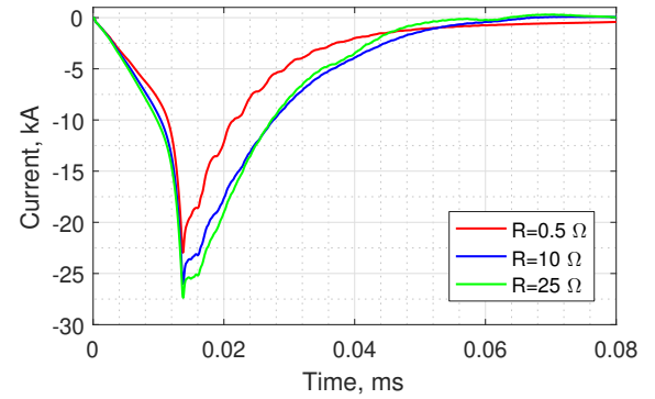
Fig. 9. Comparison of currents conducted by the SPD in phase C at generator terminals, for grounding resistances 0.5 \Omega , 10 \Omega and 25 \Omega
