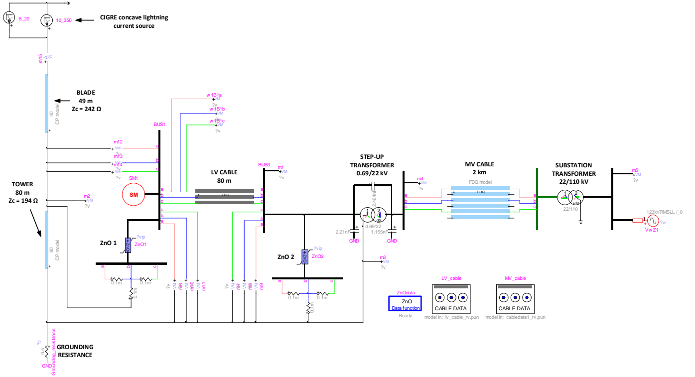
Fig. 3. EMTP-RV model of a lightning strike to a wind turbine blade
