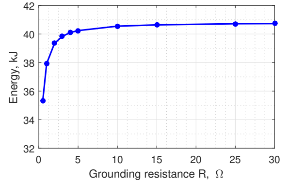
Fig. 13. Energy absorption of the SPD in phase C at generator terminals, in case of 10/350 \mu s strike, with respect to grounding resistance
