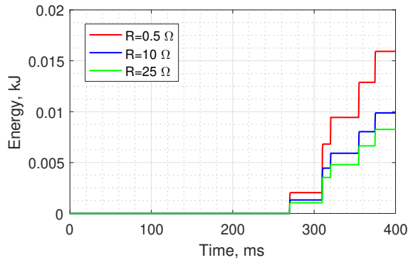
Fig. 15. Energy absorption of the SPD in phase C at generator terminals LV side of the step-up transformer in case of combined ICC and subsequent lightning strikes
