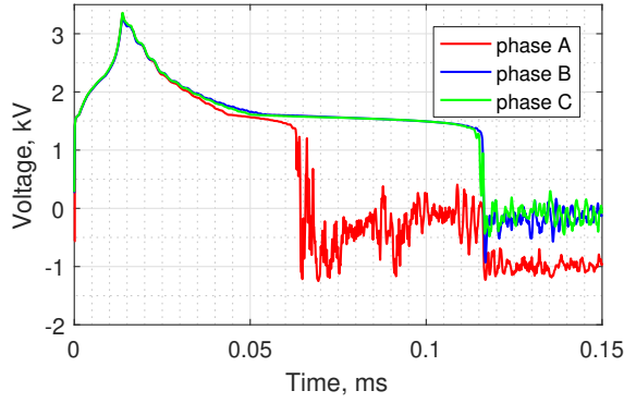
Fig. 5. Voltage at the generator with SPD protection, U_{max} = 3.3 kV
