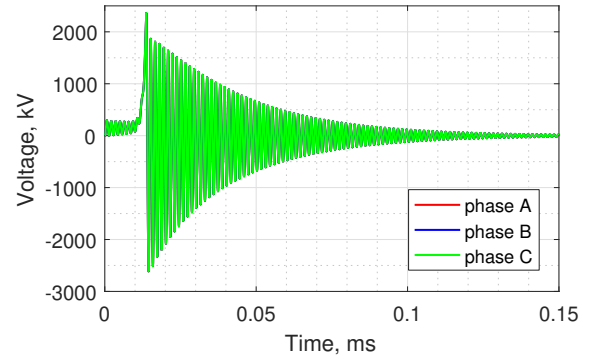
Fig. 4. Voltage at the generator without the SPD protection, U_{max} = -2703 kV
