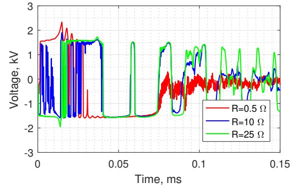
Fig. 8. Comparison of the overvoltages at the LV transformer side in phase C, in case of 8/20 \mu s strike, for grounding resistances 0.5 \Omega , 10 \Omega and 25 \Omega
