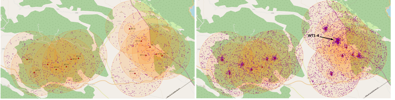
Fig. 2. Map of the WPP location with visible strikes before (left) and after the wind turbines installation (right)
