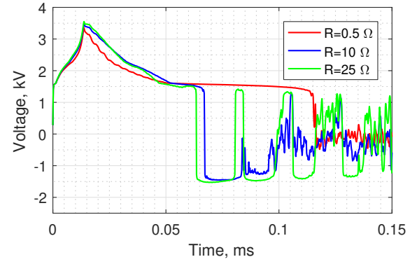
Fig. 7. Comparison of the overvoltages at the generator in phase C, in case of 8/20 \mu s strike, for grounding resistances 0.5 \Omega , 10 \Omega and 25 \Omega
