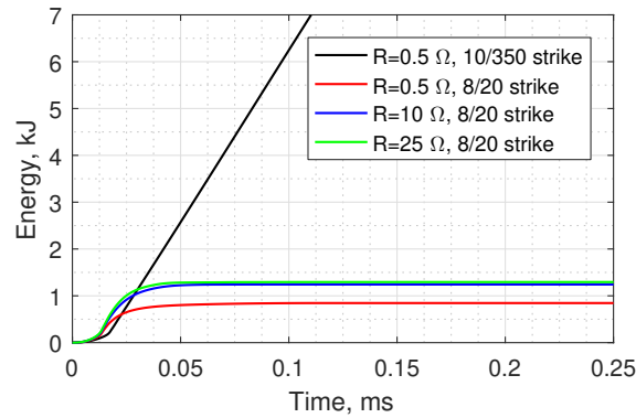
Fig. 11. Energy absorption of the SPD in phase C at generator terminals, for 8/20 \mu s and 10/350 \mu s strikes and grounding resistances 0.5 \Omega , 10 \Omega and 25 \Omega
