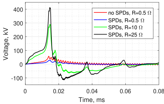
Fig. 6. Transient ground potential rise comparison in case of 8/20 \mu s , 100 kA strike, for grounding resistances 0.5 \Omega , 10 \Omega and 25 \Omega
