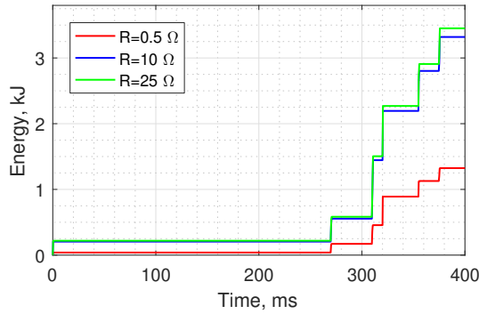
Fig. 14. Energy absorption of the SPD in phase C at generator terminals, in case of combined ICC and subsequent lightning strikes
