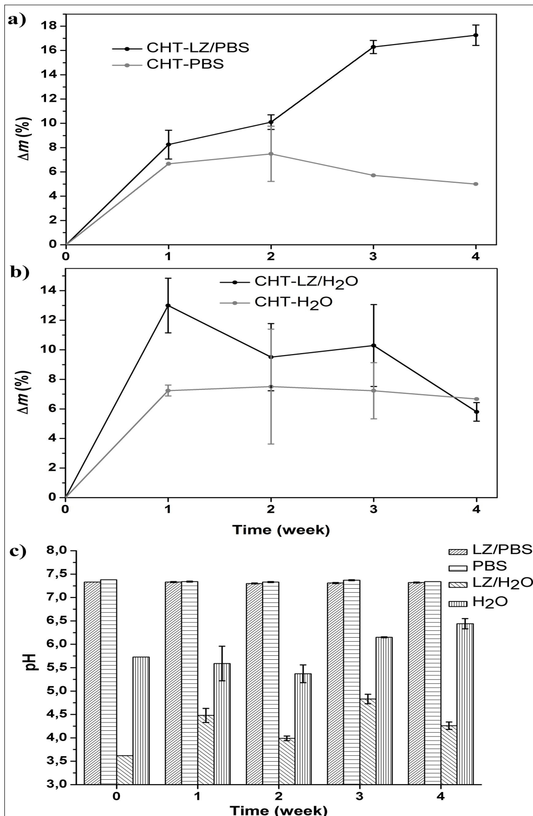
Figure 4. Degradation ratio of chitosan scaffolds performed in phosphate buffer saline solution a) and water b); the pH of incubation medium during degradation c).
