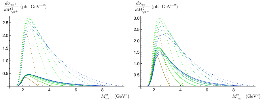
Fig. 3. Left: Differential cross section d\sigma/dM_{\gamma\pi^+}^2 for the production of a photon and a \pi^+ meson on a proton target. Right: Differential cross section d\sigma/dM_{\gamma\pi^-}^2 for the production of a photon and a \pi^- meson on a neutron target. The values of S_{\gamma N} vary in the set 8, 10, 12, 14, 16, 18, 20 \text{GeV}^2 . (from 8: left, brown to 20: right, blue), covering the JLab energy range. We use here the “valence” (solid) and the “standard” (dotted) scenarios.
