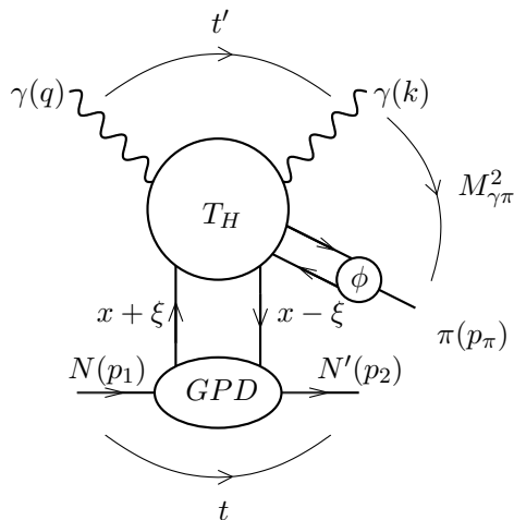
Fig. 1. Factorization of the amplitude for \gamma + N \rightarrow \gamma + \pi + N' at large M_{\gamma\pi}^2 .
