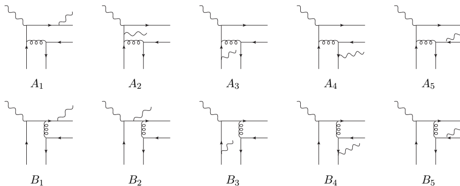
Fig. 2. Half of the Feynman diagrams contributing to the hard amplitude.
