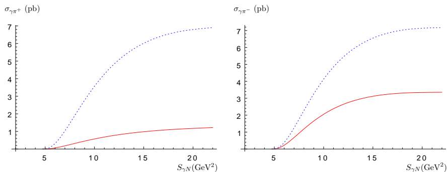
Fig. 4. Left: Integrated cross section for the production of a large mass \gamma\pi^+ pair on a proton target. Right: Integrated cross section for the production of a large mass \gamma\pi^- pair on a neutron target. The solid red curves correspond to the “valence” scenario while the dotted blue curves correspond to the “standard” one.
