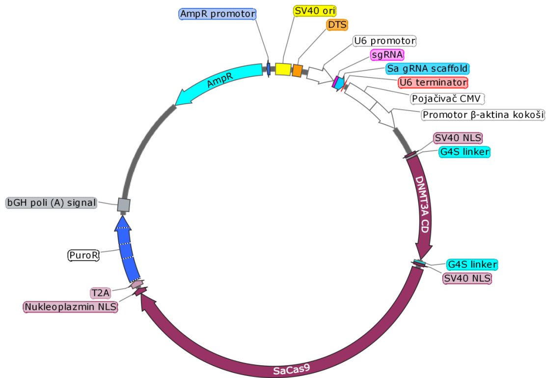
pN-DNMT3a/SaCas9/Puro/sgRNA 8539 bp
