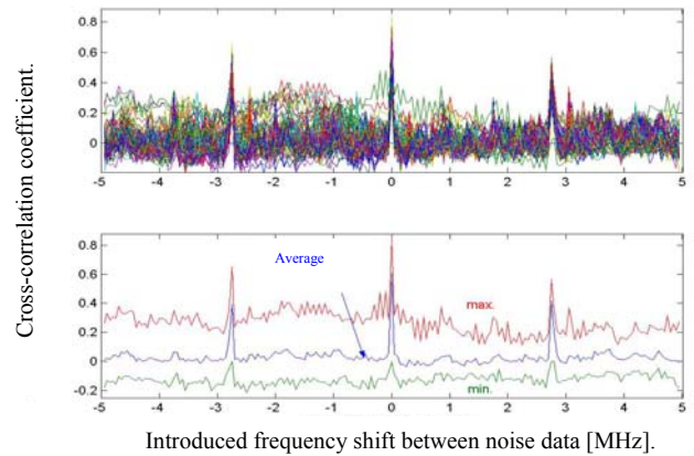
Fig. 12. Crosscorrelation functions with respect to frequency shift for all possible pairs of "unit" noise samples taken at the same network terminal, but at 15 different times, in one-hour raster. Lower diagram shows for clarity only average, minimum and maximum values. Compare with Fig. 11.
