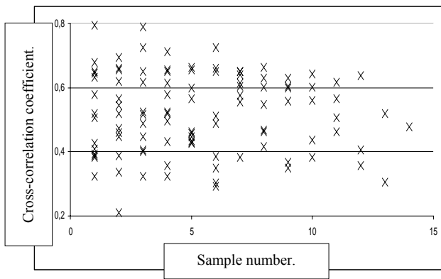
Fig. 9. Cross-correlation coefficients for all possible pairs of noise samples taken at 15 different network terminals during 10 minutes (i.e. approximately at the same time). Note that coefficients are in average quite high valued.
