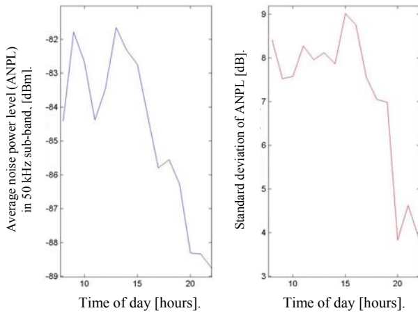
Fig. 6. Example of daily variation in average noise power level and its standard deviation. Office building, same working day as in Fig. 5, 5 minutes maximum data.
