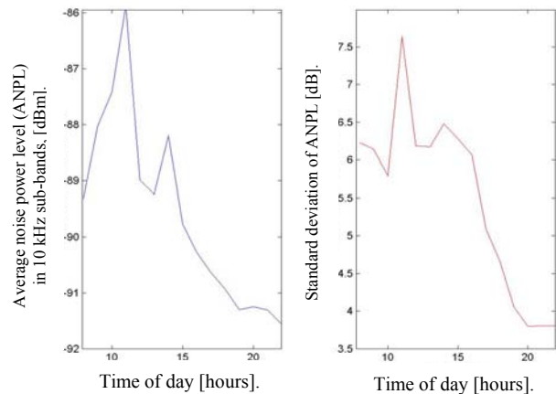
Fig. 5. Example of daily variation in average noise power level and its standard deviation. Office building, working day, one-scan data.
