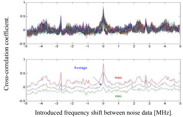
Fig. 11. Crosscorrelation functions with respect to frequency shift for all possible pairs of noise samples taken at the same network terminal, but at 15 different times, in one-hour raster. Lower diagram shows for clarity only average, minimum and maximum values.
