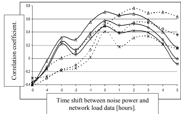
Fig. 8. Correlation functions between electrical load and noise power. Solid: one-scan data; dashed: 5 minutes maximums. Triangle: strong narrowband noise components; rhomboid: total noise; cross: floor noise (i.e. components weaker than P_0 ). The q^* value for both one-scan and 5 minutes maximum data is 18.8 dB.
