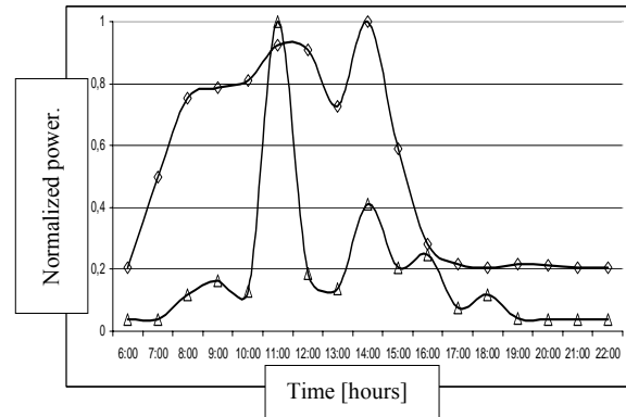
Fig. 7. Normalized electrical load and noise power in office building. Triangle: noise. Rhomboid: network electrical load. Scale is linear (not log).
