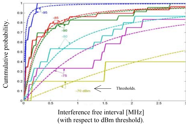
Fig. 4. Example of cumulative distributions of the band width of interference free intervals with respect to certain power level threshold. This is the probability that the frequency interval within which the noise level is lower or equal to threshold is less or equal to the abscissa value.
