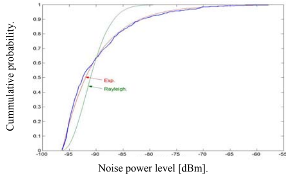
Fig.2. An example of cumulative probability of noise power levels in a frequency band from 10 to 30 MHz. Residential house, working day, noon.
